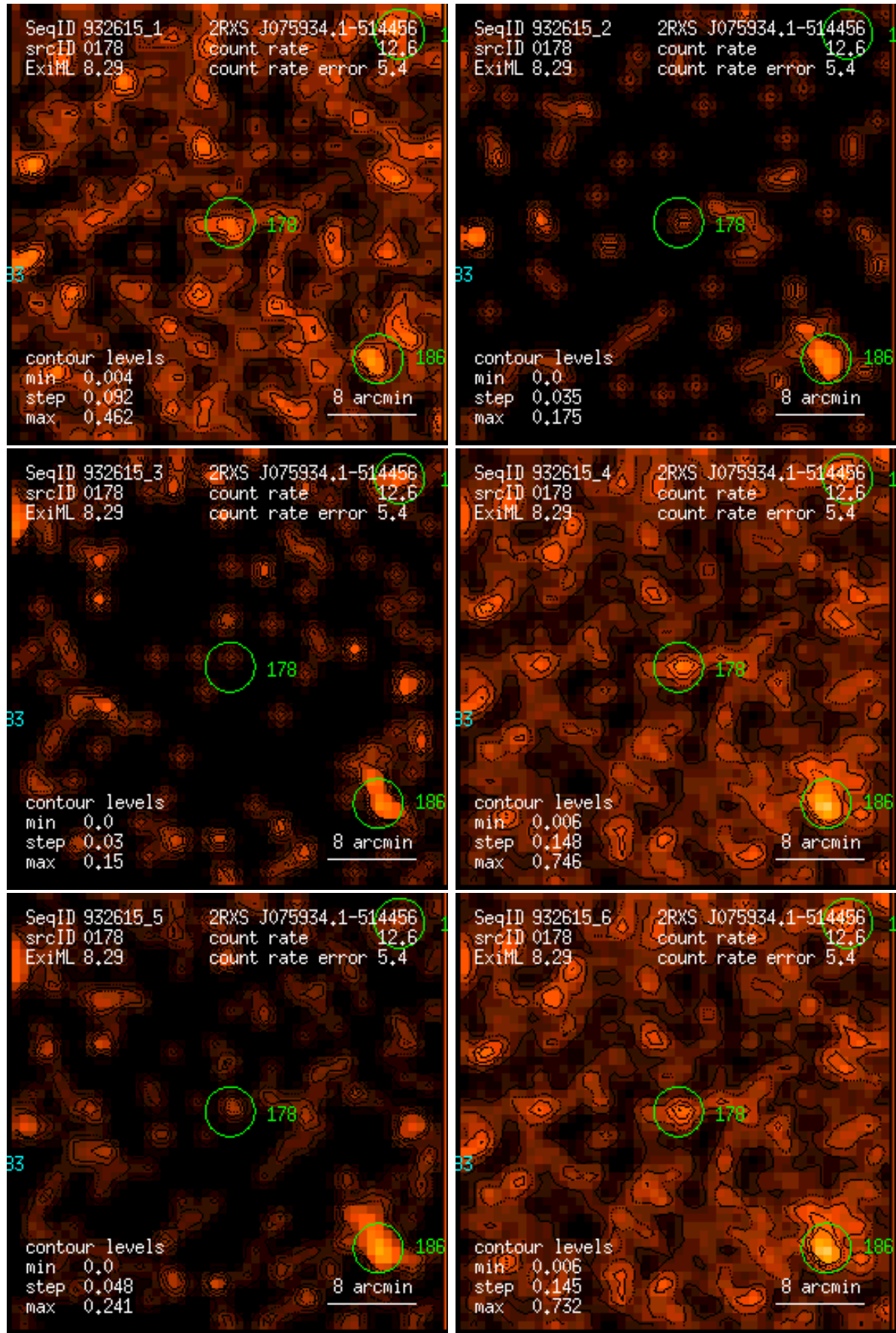
Figure 178: RASS 932615: detection 0178: band rate images, Gaussian filter: (1) PSPC channels 11 – 41, (2) 52 – 90, (3) 91 – 201, (4) 11 – 235, (5) 52 – 201, (6) 11 – 201. Broad band rates in counts/ks. Band rate contour levels in counts/ks/arcmin 2 .
