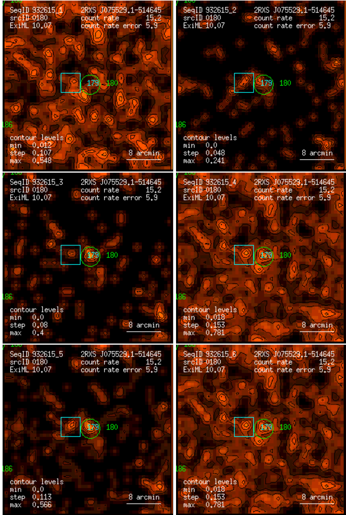
Figure 180: RASS 932615: detection 0180: band rate images, Gaussian filter: (1) PSPC channels 11 – 41, (2) 52 – 90, (3) 91 – 201, (4) 11 – 235, (5) 52 – 201, (6) 11 – 201. Broad band rates in counts/ks. Band rate contour levels in counts/ks/arcmin 2 .
