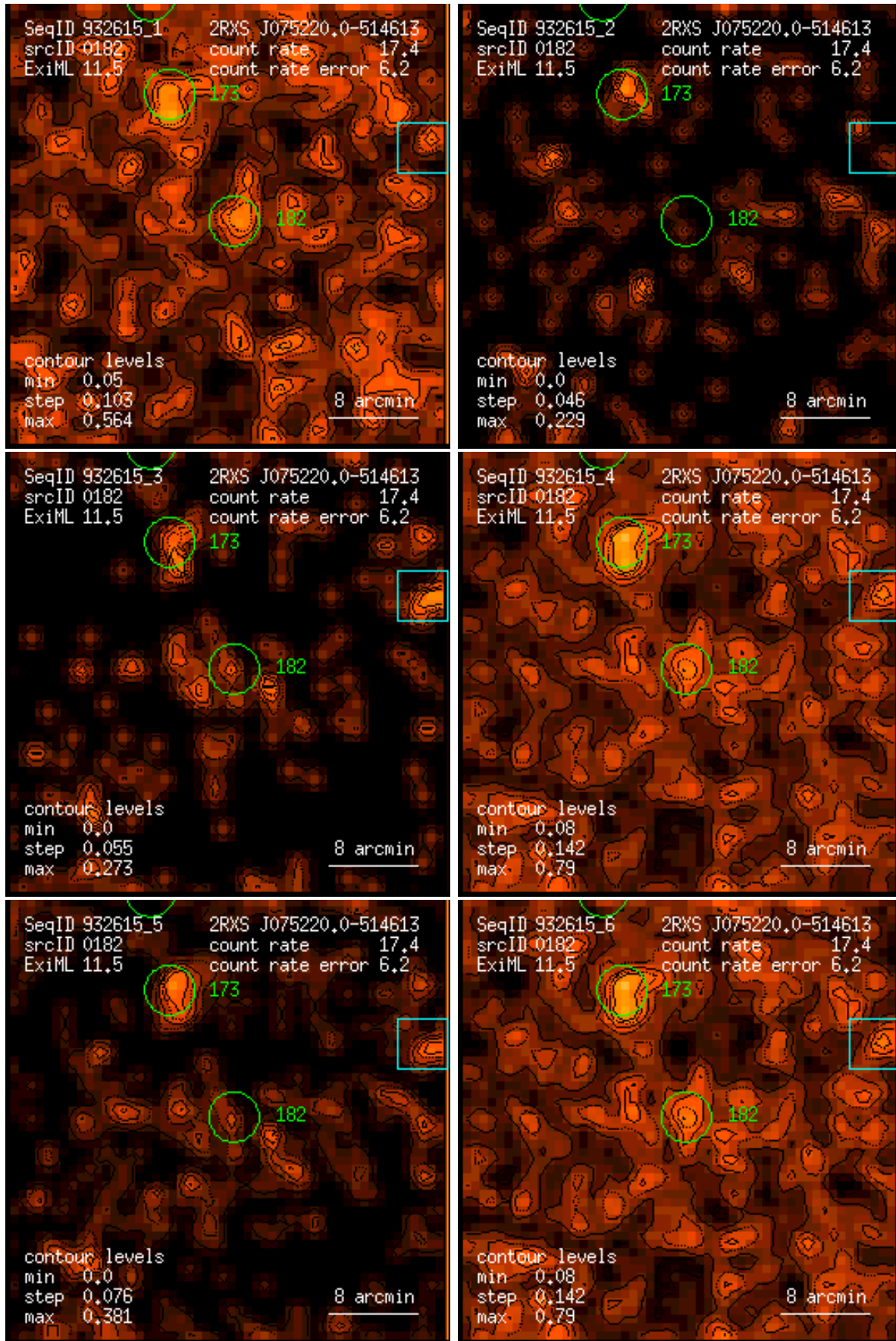
Figure 182: RASS 932615: detection 0182: band rate images, Gaussian filter: (1) PSPC channels 11 – 41, (2) 52 – 90, (3) 91 – 201, (4) 11 – 235, (5) 52 – 201, (6) 11 – 201. Broad band rates in counts/ks. Band rate contour levels in counts/ks/arcmin 2 .
