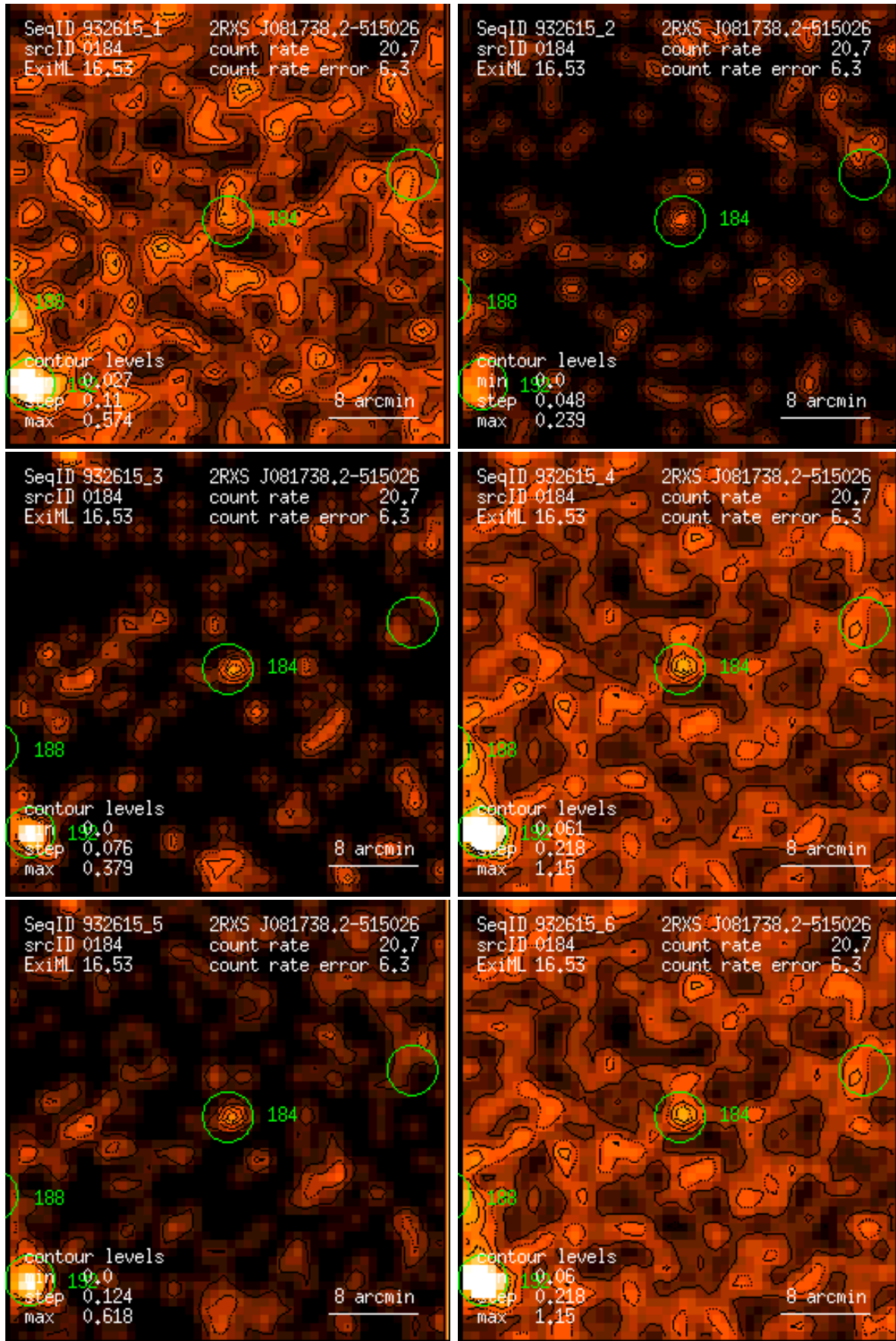
Figure 184: RASS 932615: detection 0184: band rate images, Gaussian filter: (1) PSPC channels 11 – 41, (2) 52 – 90, (3) 91 – 201, (4) 11 – 235, (5) 52 – 201, (6) 11 – 201. Broad band rates in counts/ks. Band rate contour levels in counts/ks/arcmin 2 .
