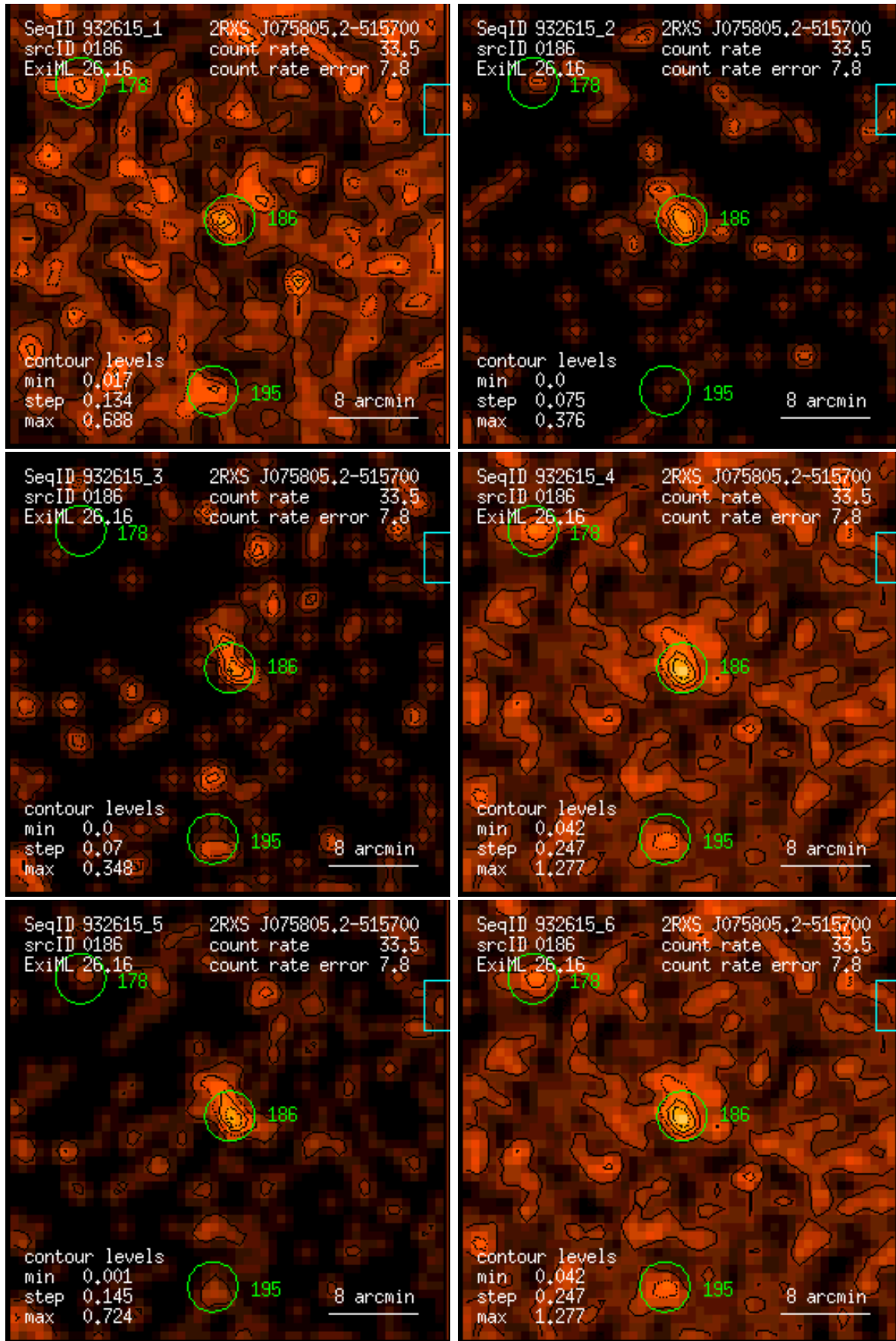
Figure 186: RASS 932615: detection 0186: band rate images, Gaussian filter: (1) PSPC channels 11 – 41, (2) 52 – 90, (3) 91 – 201, (4) 11 – 235, (5) 52 – 201, (6) 11 – 201. Broad band rates in counts/ks. Band rate contour levels in counts/ks/arcmin 2 .
