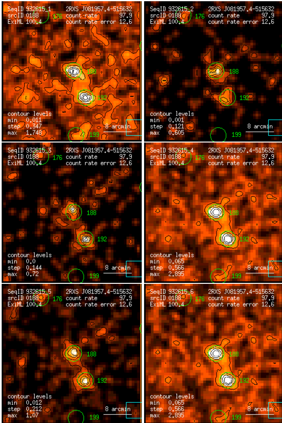
Figure 188: RASS 932615: detection 0188: band rate images, Gaussian filter: (1) PSPC channels 11 – 41, (2) 52 – 90, (3) 91 – 201, (4) 11 – 235, (5) 52 – 201, (6) 11 – 201. Broad band rates in counts/ks. Band rate contour levels in counts/ks/arcmin 2 .
