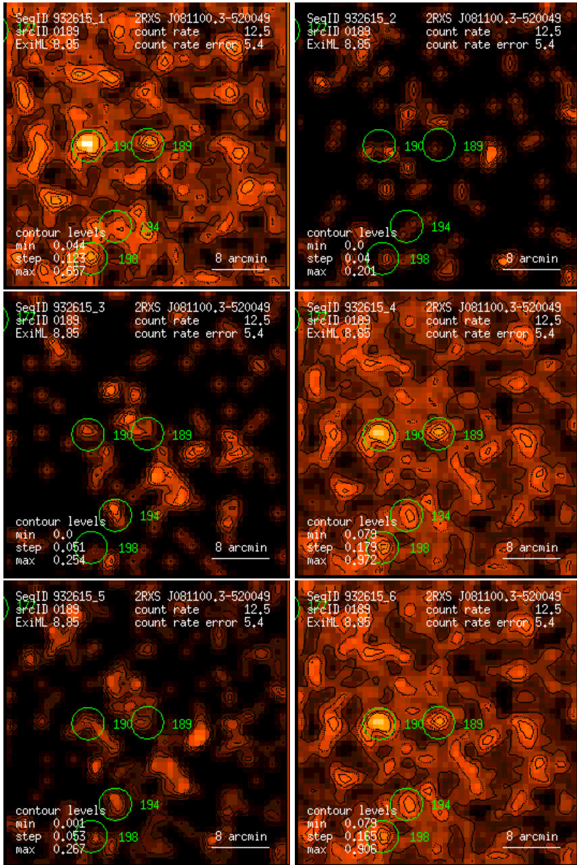
Figure 189: RASS 932615: detection 0189: band rate images, Gaussian filter: (1) PSPC channels 11 – 41, (2) 52 – 90, (3) 91 – 201, (4) 11 – 235, (5) 52 – 201, (6) 11 – 201. Broad band rates in counts/ks. Band rate contour levels in counts/ks/arcmin 2 .
