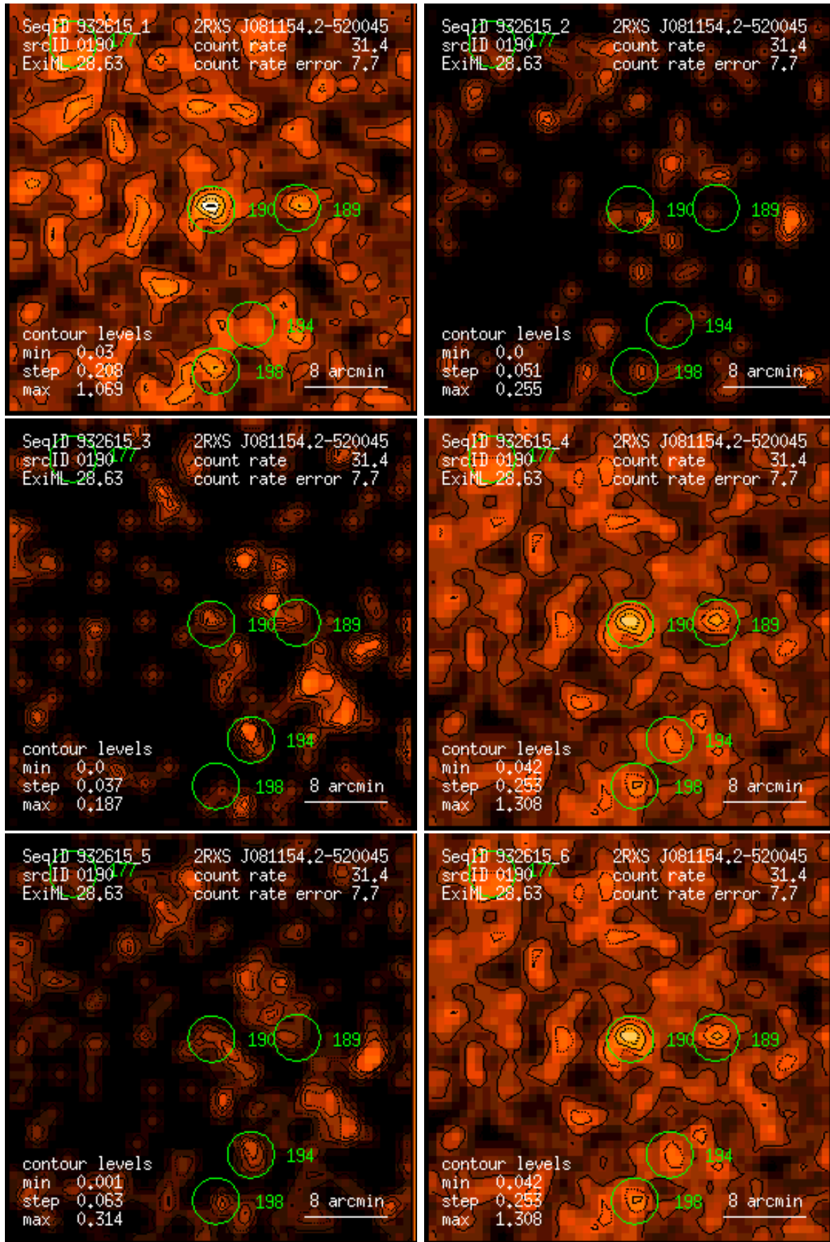
Figure 190: RASS 932615: detection 0190: band rate images, Gaussian filter: (1) PSPC channels 11 – 41, (2) 52 – 90, (3) 91 – 201, (4) 11 – 235, (5) 52 – 201, (6) 11 – 201. Broad band rates in counts/ks. Band rate contour levels in counts/ks/arcmin 2 .
