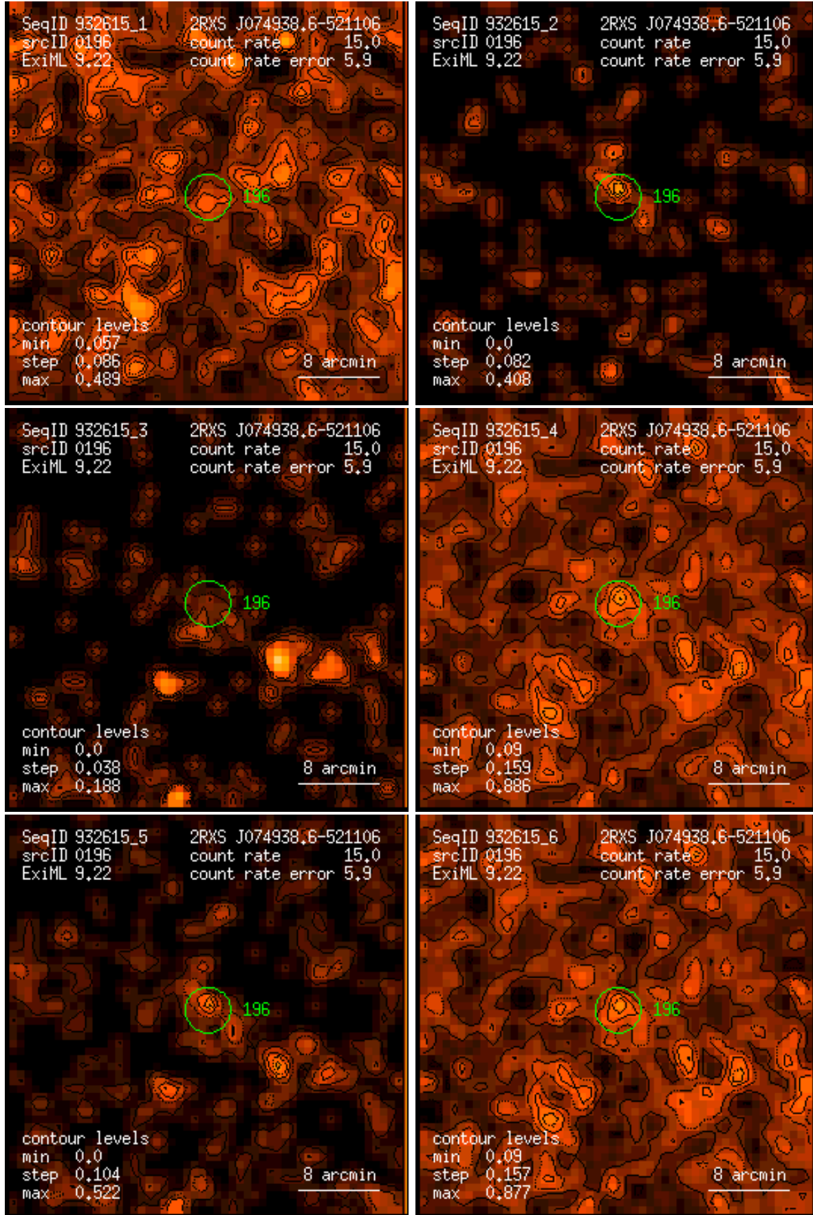
Figure 196: RASS 932615: detection 0196: band rate images, Gaussian filter: (1) PSPC channels 11 – 41, (2) 52 – 90, (3) 91 – 201, (4) 11 – 235, (5) 52 – 201, (6) 11 – 201. Broad band rates in counts/ks. Band rate contour levels in counts/ks/arcmin 2 .
