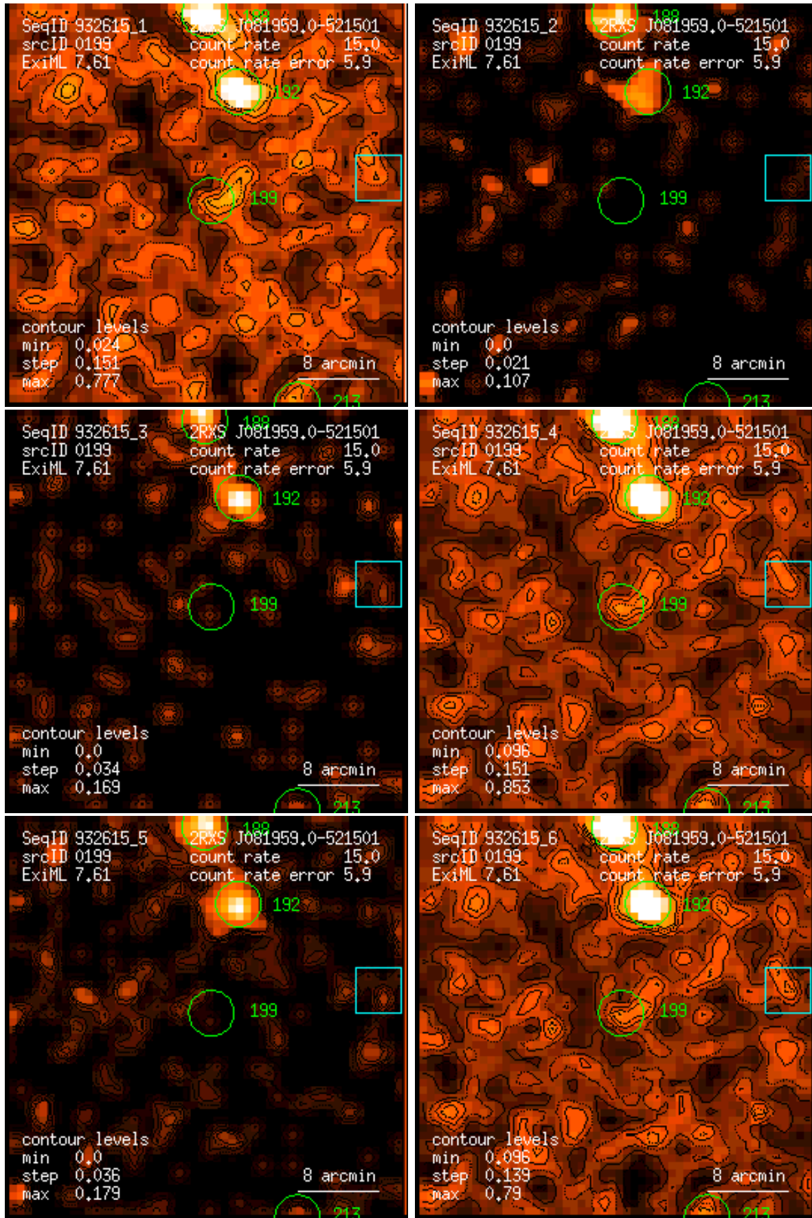
Figure 199: RASS 932615: detection 0199: band rate images, Gaussian filter: (1) PSPC channels 11 – 41, (2) 52 – 90, (3) 91 – 201, (4) 11 – 235, (5) 52 – 201, (6) 11 – 201. Broad band rates in counts/ks. Band rate contour levels in counts/ks/arcmin 2 .
