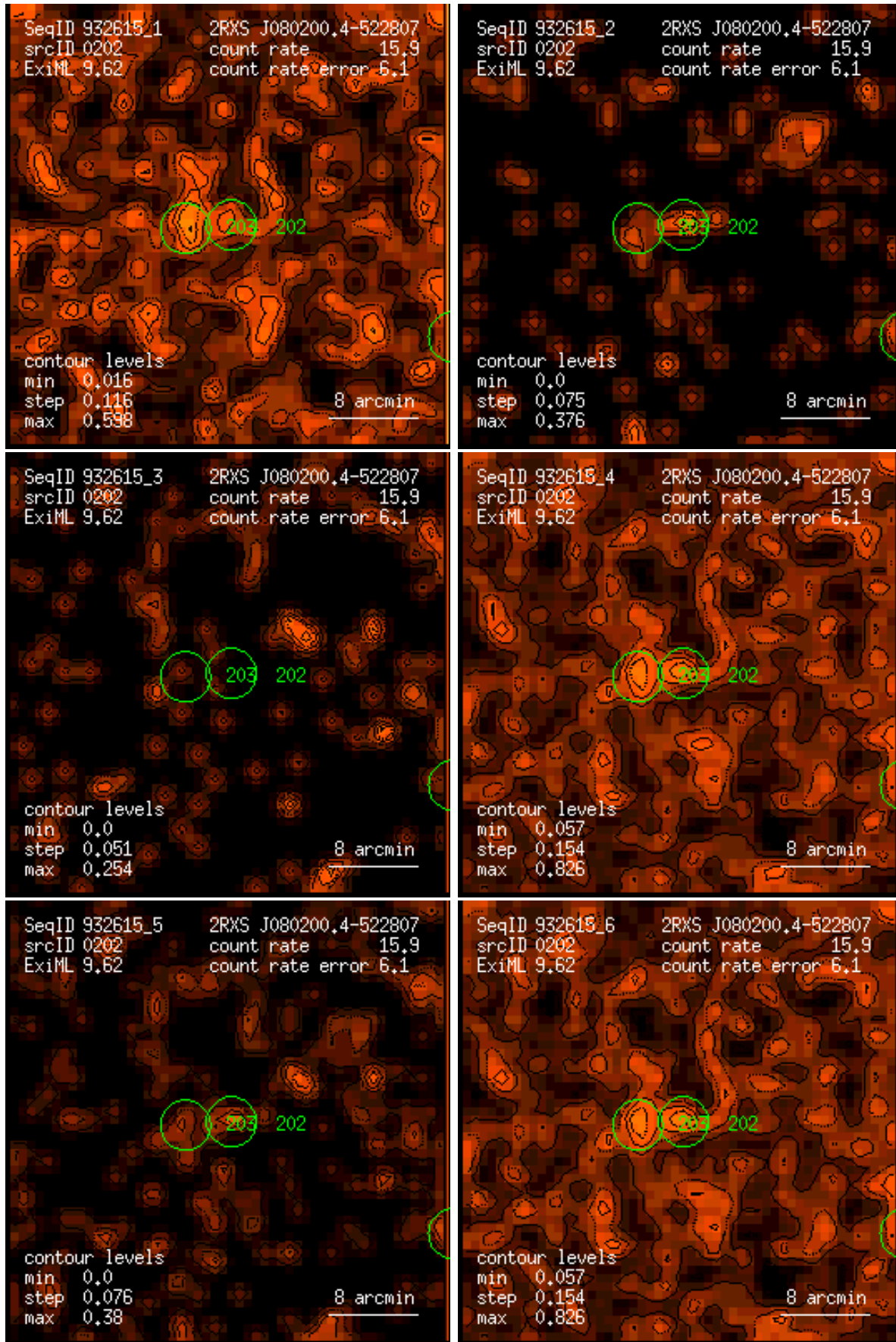
Figure 202: RASS 932615: detection 0202: band rate images, Gaussian filter: (1) PSPC channels 11 – 41, (2) 52 – 90, (3) 91 – 201, (4) 11 – 235, (5) 52 – 201, (6) 11 – 201. Broad band rates in counts/ks. Band rate contour levels in counts/ks/arcmin 2 .
