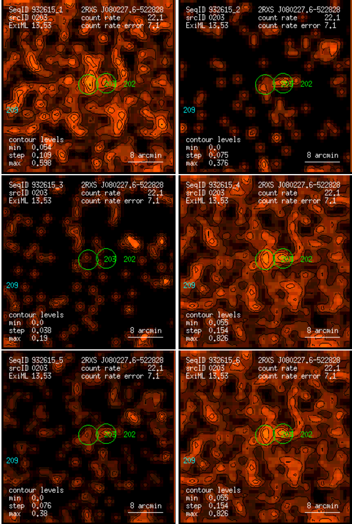
Figure 203: RASS 932615: detection 0203: band rate images, Gaussian filter: (1) PSPC channels 11 – 41, (2) 52 – 90, (3) 91 – 201, (4) 11 – 235, (5) 52 – 201, (6) 11 – 201. Broad band rates in counts/ks. Band rate contour levels in counts/ks/arcmin 2 .
