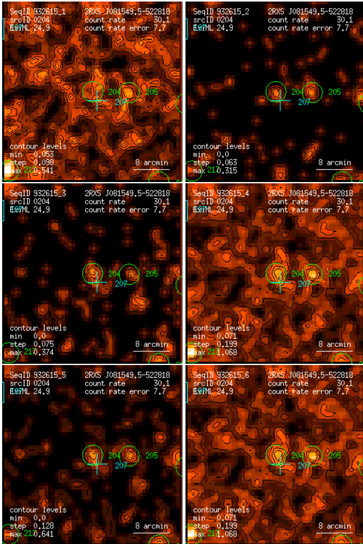
Figure 204: RASS 932615: detection 0204: band rate images, Gaussian filter: (1) PSPC channels 11 – 41, (2) 52 – 90, (3) 91 – 201, (4) 11 – 235, (5) 52 – 201, (6) 11 – 201. Broad band rates in counts/ks. Band rate contour levels in counts/ks/arcmin 2 .
