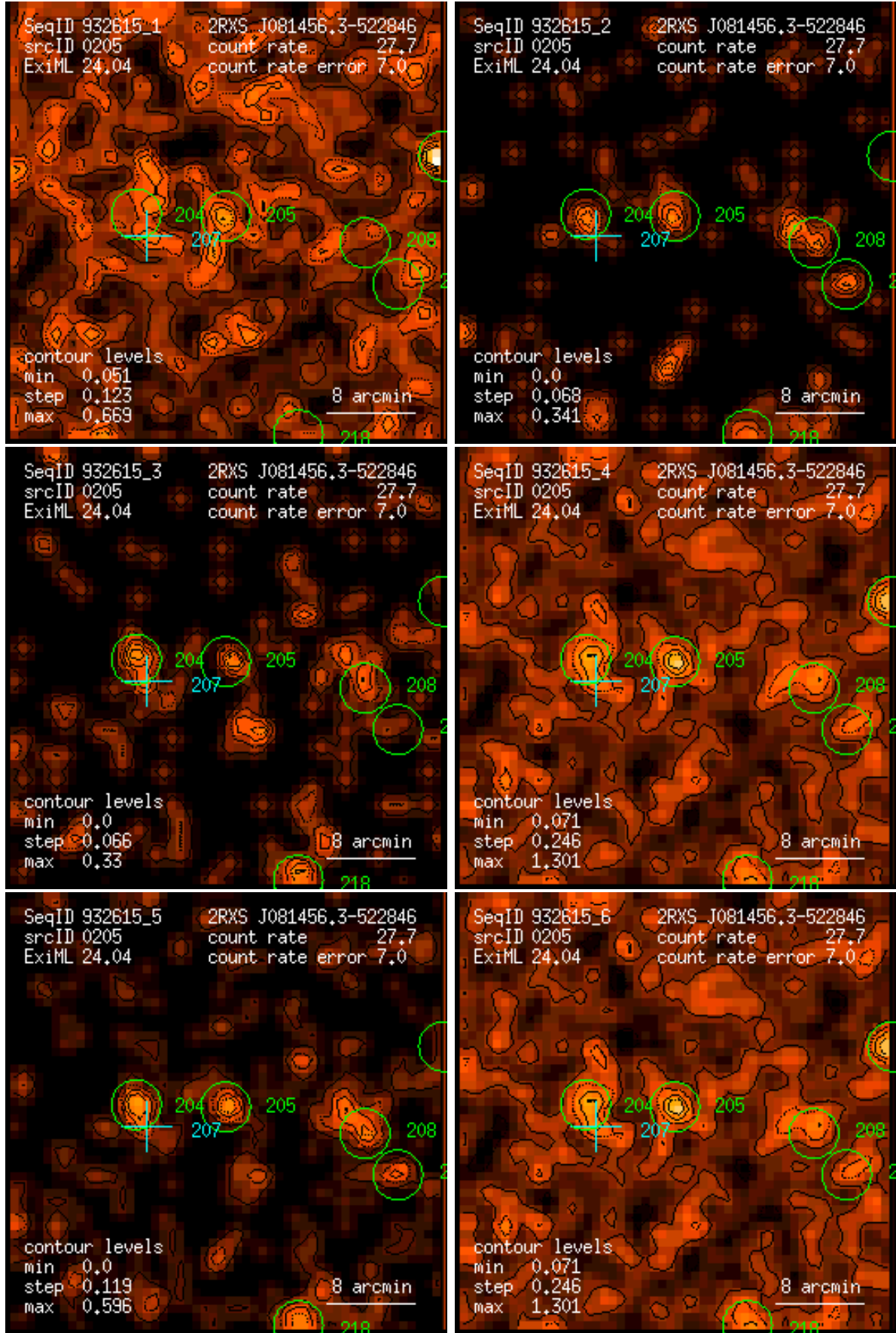
Figure 205: RASS 932615: detection 0205: band rate images, Gaussian filter: (1) PSPC channels 11 – 41, (2) 52 – 90, (3) 91 – 201, (4) 11 – 235, (5) 52 – 201, (6) 11 – 201. Broad band rates in counts/ks. Band rate contour levels in counts/ks/arcmin 2 .
