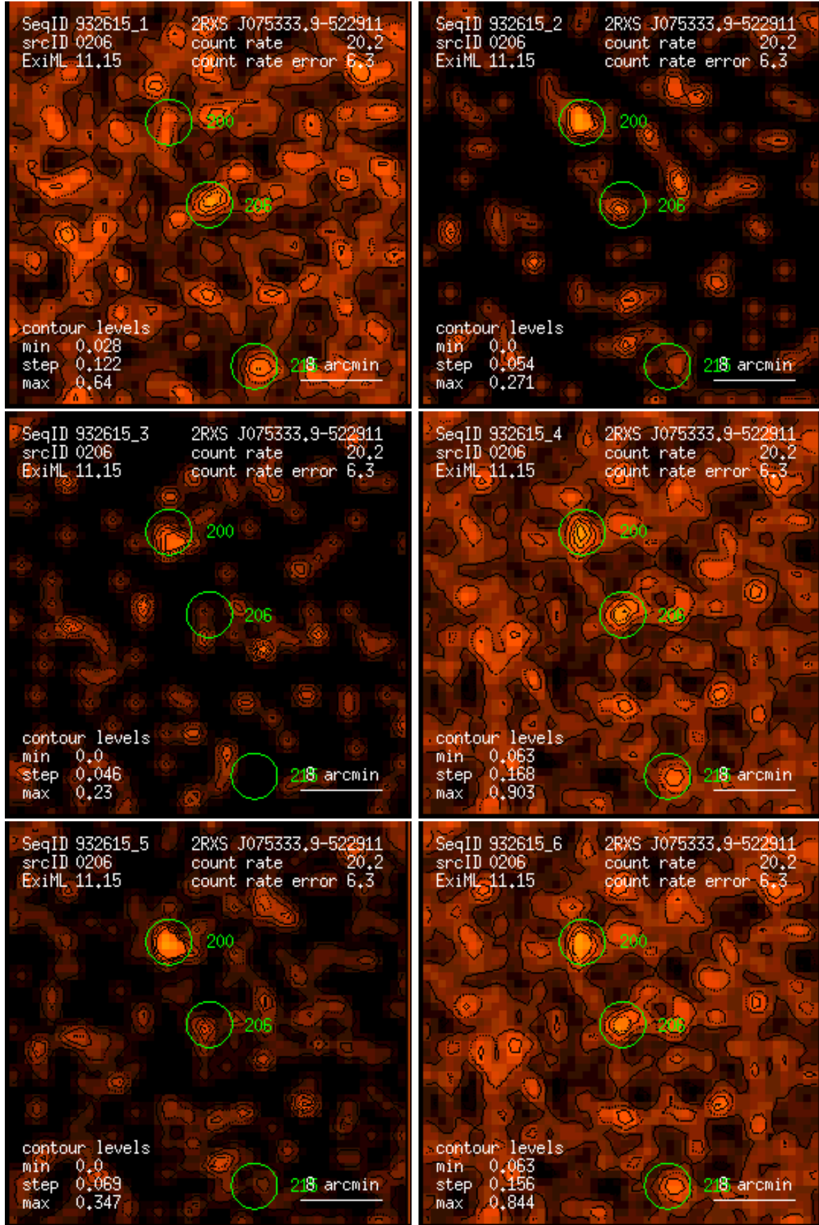
Figure 206: RASS 932615: detection 0206: band rate images, Gaussian filter: (1) PSPC channels 11 – 41, (2) 52 – 90, (3) 91 – 201, (4) 11 – 235, (5) 52 – 201, (6) 11 – 201. Broad band rates in counts/ks. Band rate contour levels in counts/ks/arcmin 2 .
