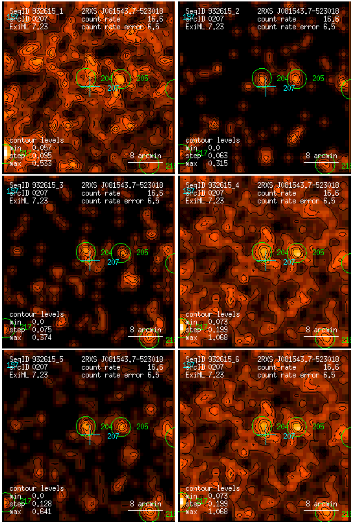
Figure 207: RASS 932615: detection 0207: band rate images, Gaussian filter: (1) PSPC channels 11 – 41, (2) 52 – 90, (3) 91 – 201, (4) 11 – 235, (5) 52 – 201, (6) 11 – 201. Broad band rates in counts/ks. Band rate contour levels in counts/ks/arcmin 2 .
