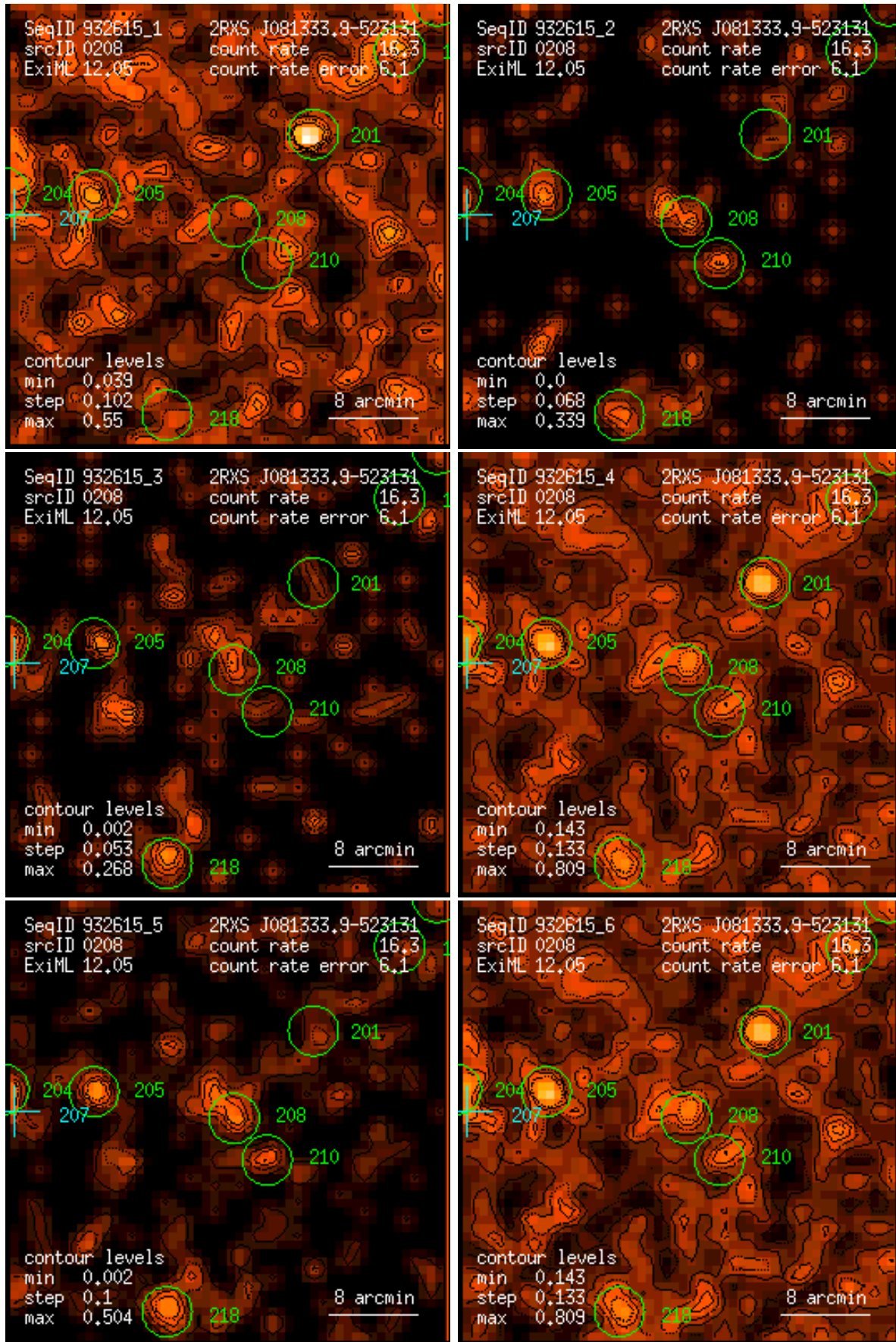
Figure 208: RASS 932615: detection 0208: band rate images, Gaussian filter: (1) PSPC channels 11 – 41, (2) 52 – 90, (3) 91 – 201, (4) 11 – 235, (5) 52 – 201, (6) 11 – 201. Broad band rates in counts/ks. Band rate contour levels in counts/ks/arcmin 2 .
