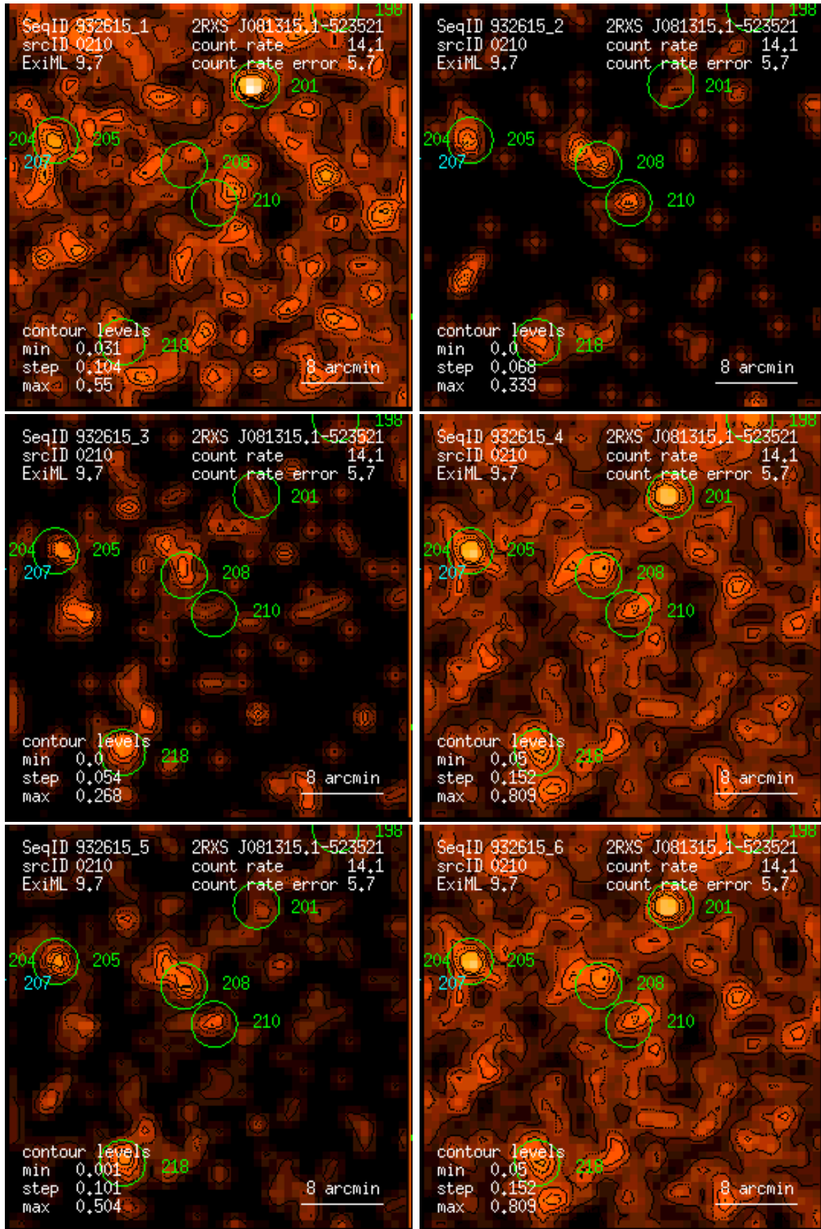
Figure 210: RASS 932615: detection 0210: band rate images, Gaussian filter: (1) PSPC channels 11 – 41, (2) 52 – 90, (3) 91 – 201, (4) 11 – 235, (5) 52 – 201, (6) 11 – 201. Broad band rates in counts/ks. Band rate contour levels in counts/ks/arcmin 2 .
