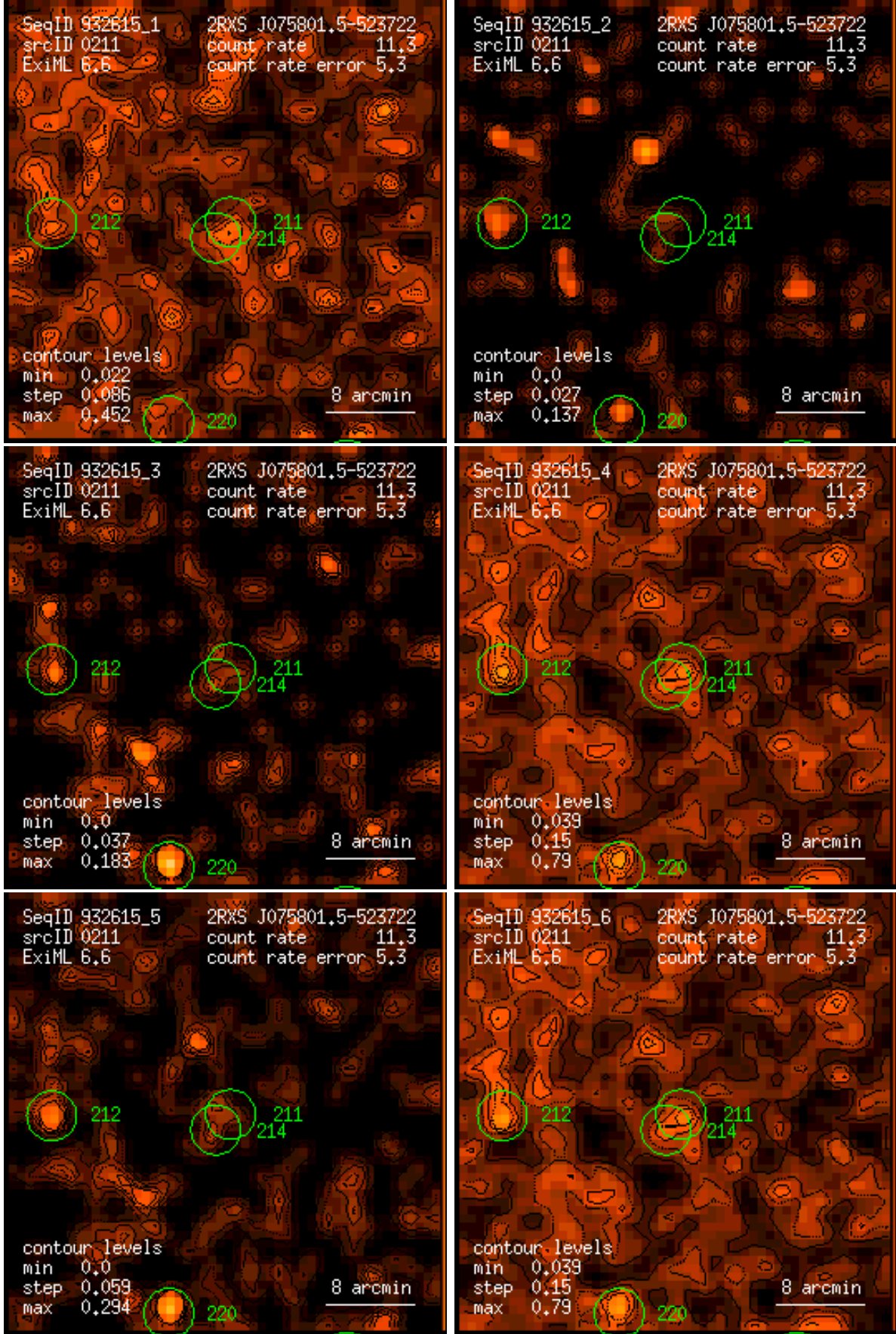
Figure 211: RASS 932615: detection 0211: band rate images, Gaussian filter: (1) PSPC channels 11 – 41, (2) 52 – 90, (3) 91 – 201, (4) 11 – 235, (5) 52 – 201, (6) 11 – 201. Broad band rates in counts/ks. Band rate contour levels in counts/ks/arcmin 2 .
