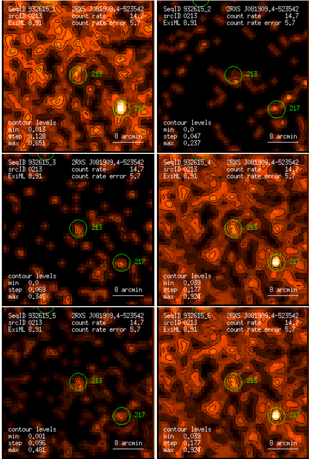
Figure 213: RASS 932615: detection 0213: band rate images, Gaussian filter: (1) PSPC channels 11 – 41, (2) 52 – 90, (3) 91 – 201, (4) 11 – 235, (5) 52 – 201, (6) 11 – 201. Broad band rates in counts/ks. Band rate contour levels in counts/ks/arcmin 2 .
