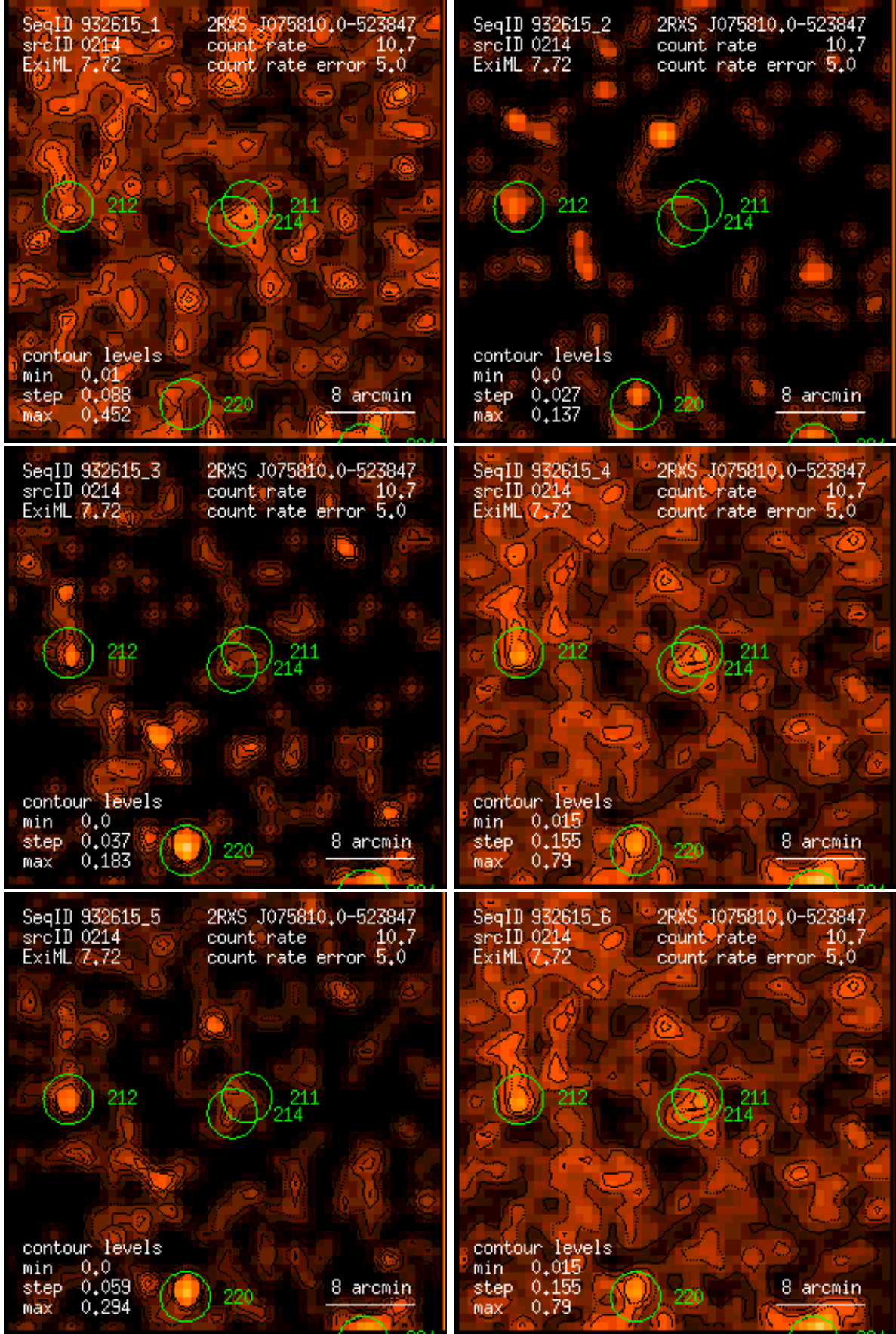
Figure 214: RASS 932615: detection 0214: band rate images, Gaussian filter: (1) PSPC channels 11 – 41, (2) 52 – 90, (3) 91 – 201, (4) 11 – 235, (5) 52 – 201, (6) 11 – 201. Broad band rates in counts/ks. Band rate contour levels in counts/ks/arcmin 2 .
