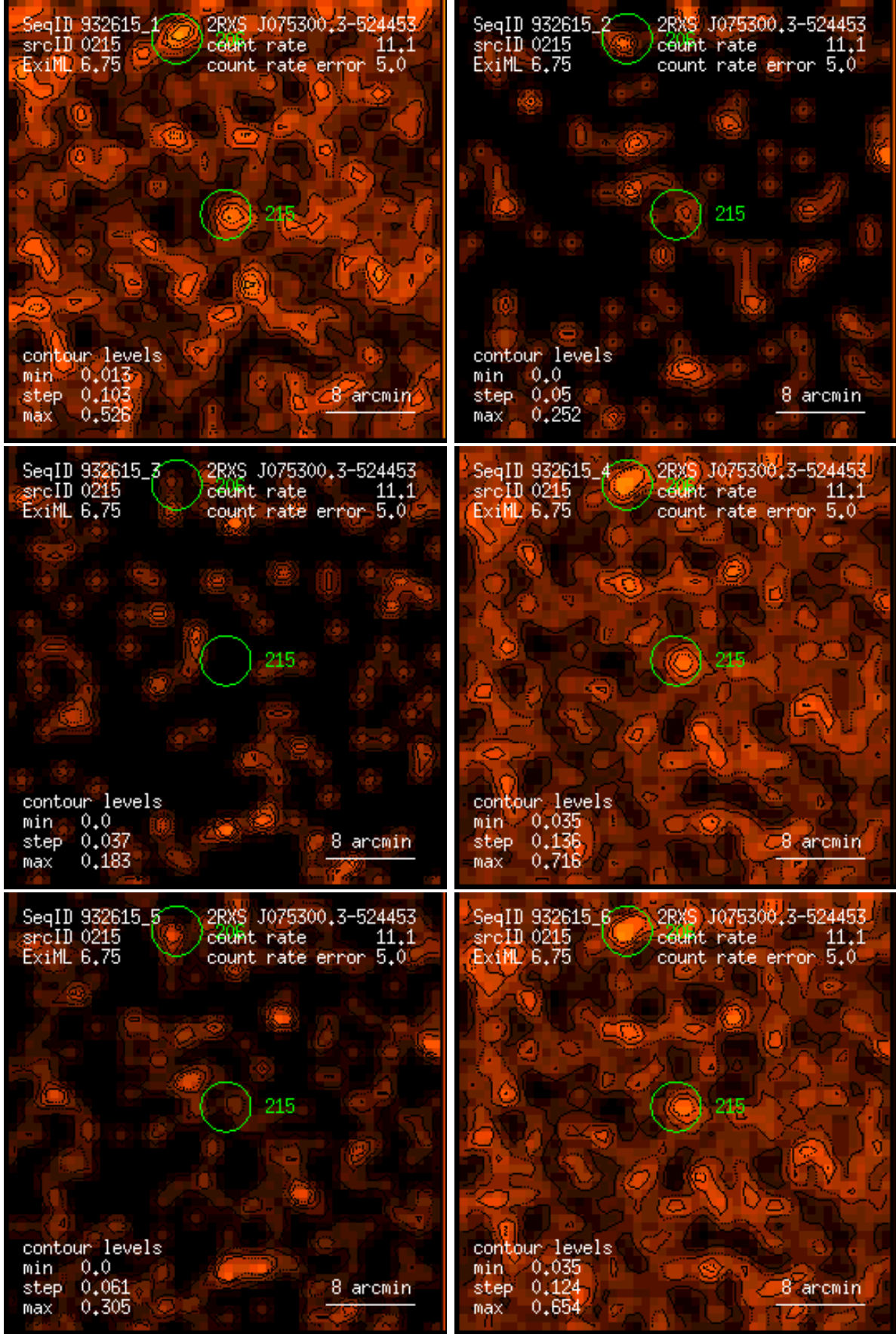
Figure 215: RASS 932615: detection 0215: band rate images, Gaussian filter: (1) PSPC channels 11 – 41, (2) 52 – 90, (3) 91 – 201, (4) 11 – 235, (5) 52 – 201, (6) 11 – 201. Broad band rates in counts/ks. Band rate contour levels in counts/ks/arcmin 2 .
