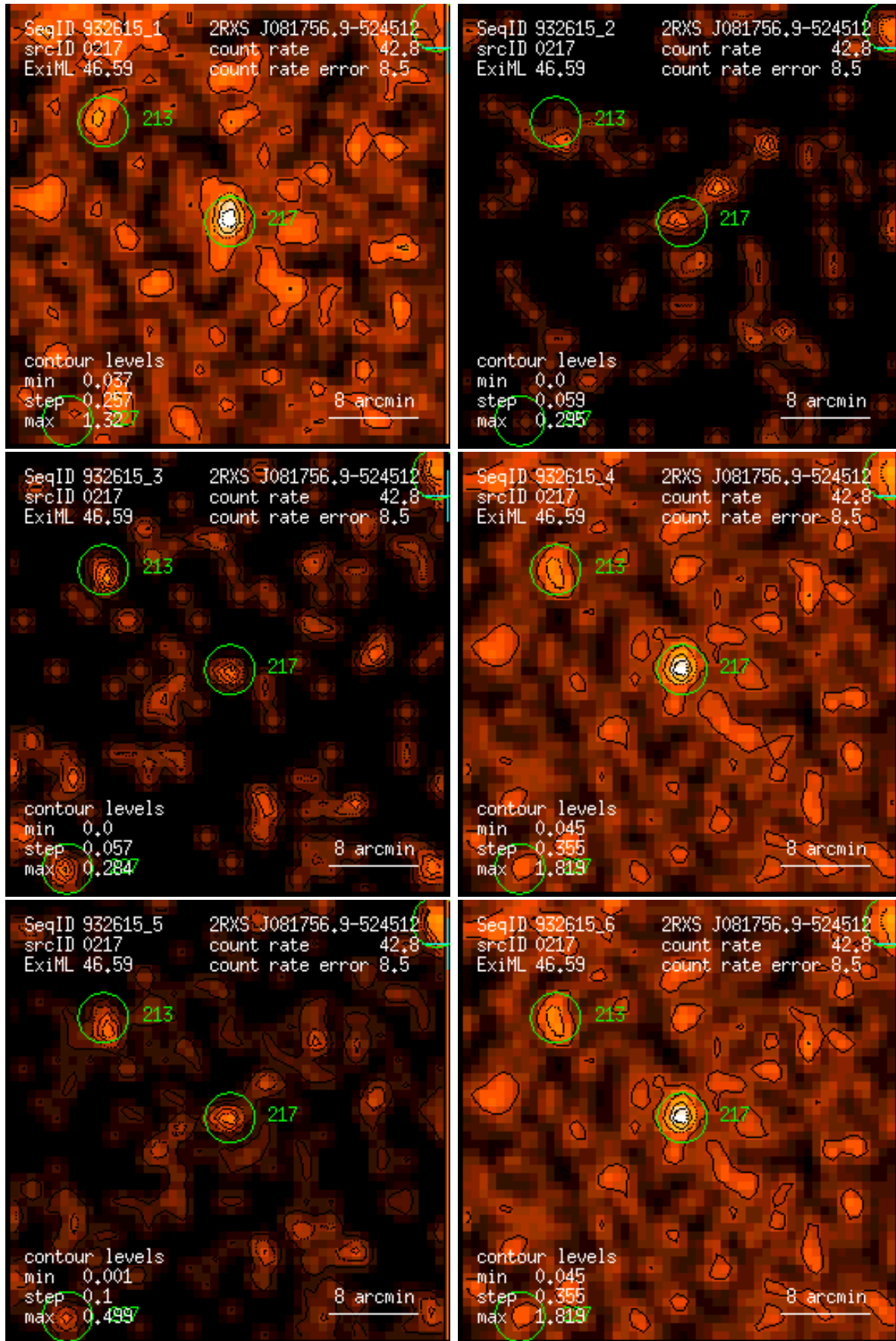
Figure 217: RASS 932615: detection 0217: band rate images, Gaussian filter: (1) PSPC channels 11 – 41, (2) 52 – 90, (3) 91 – 201, (4) 11 – 235, (5) 52 – 201, (6) 11 – 201. Broad band rates in counts/ks. Band rate contour levels in counts/ks/arcmin 2 .
