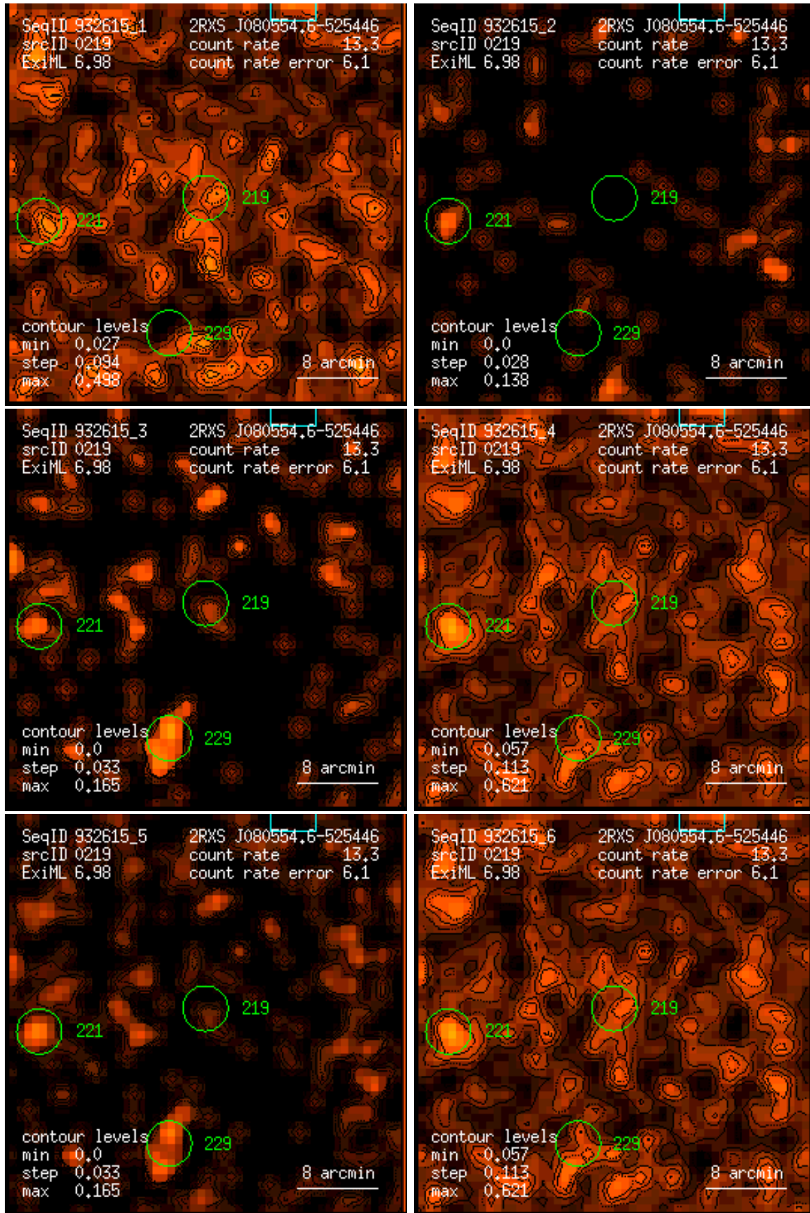
Figure 219: RASS 932615: detection 0219: band rate images, Gaussian filter: (1) PSPC channels 11 – 41, (2) 52 – 90, (3) 91 – 201, (4) 11 – 235, (5) 52 – 201, (6) 11 – 201. Broad band rates in counts/ks. Band rate contour levels in counts/ks/arcmin 2 .
