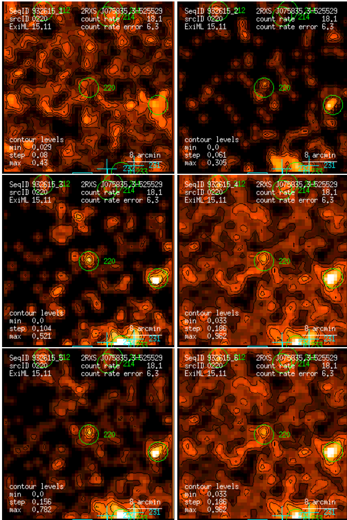
Figure 220: RASS 932615: detection 0220: band rate images, Gaussian filter: (1) PSPC channels 11 – 41, (2) 52 – 90, (3) 91 – 201, (4) 11 – 235, (5) 52 – 201, (6) 11 – 201. Broad band rates in counts/ks. Band rate contour levels in counts/ks/arcmin 2 .
