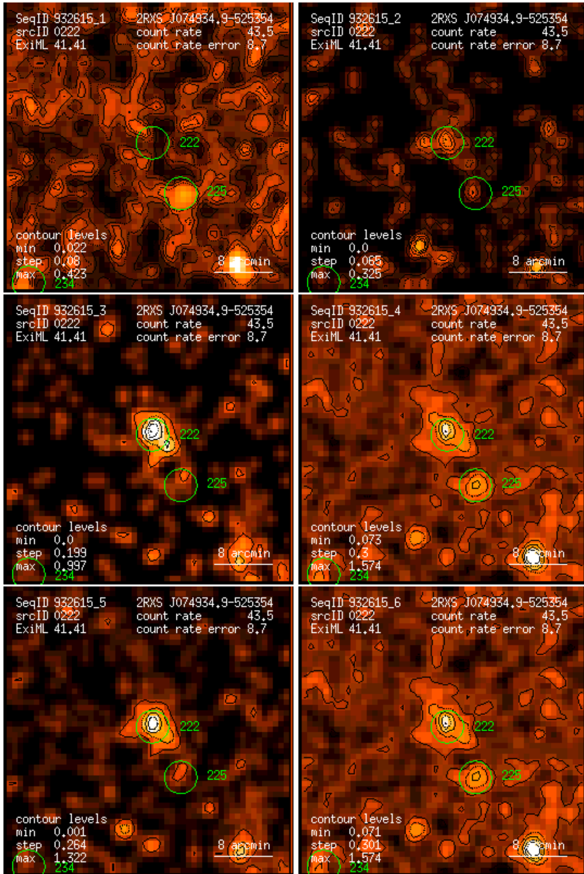
Figure 222: RASS 932615: detection 0222: band rate images, Gaussian filter: (1) PSPC channels 11 – 41, (2) 52 – 90, (3) 91 – 201, (4) 11 – 235, (5) 52 – 201, (6) 11 – 201. Broad band rates in counts/ks. Band rate contour levels in counts/ks/arcmin 2 .
