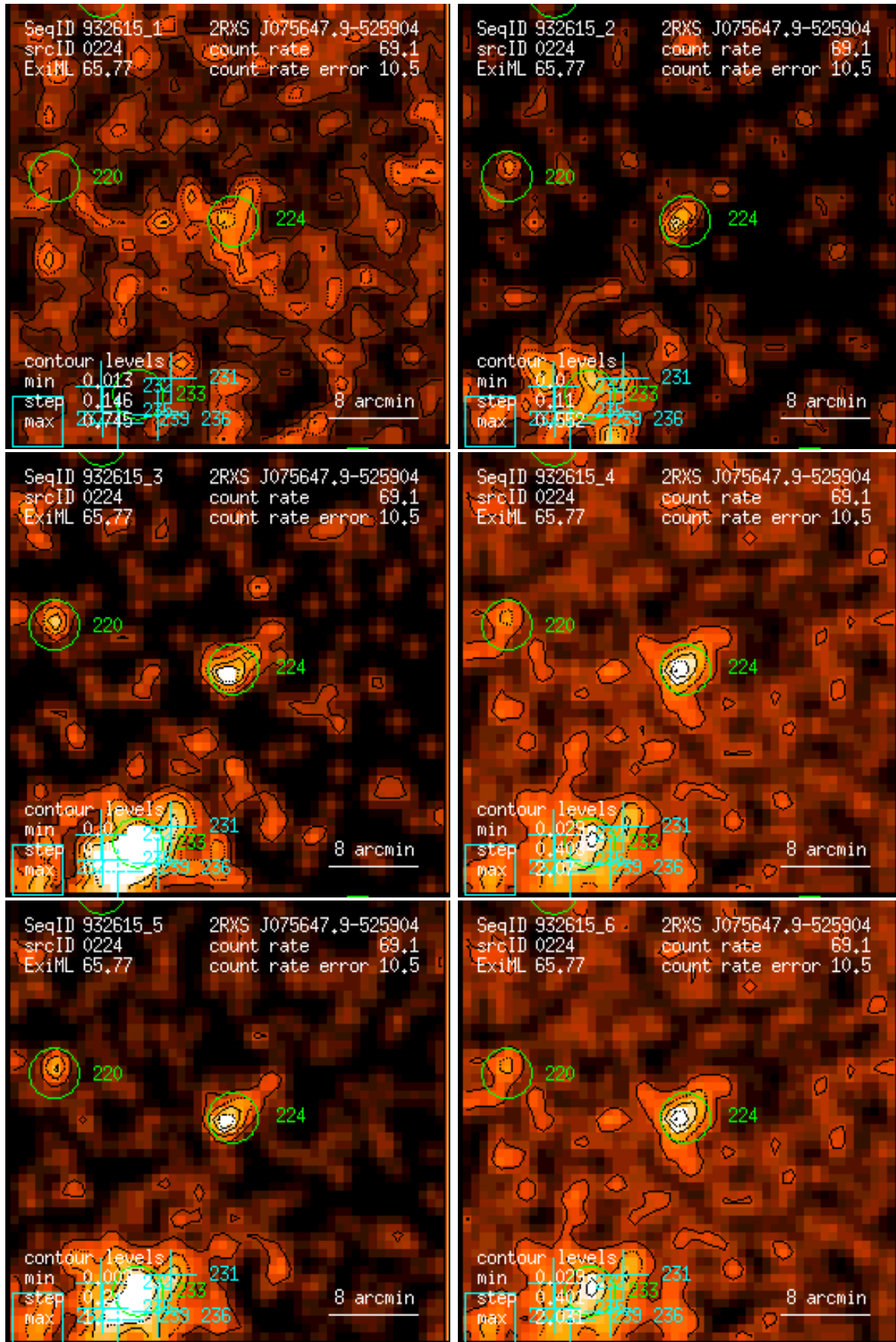
Figure 224: RASS 932615: detection 0224: band rate images, Gaussian filter: (1) PSPC channels 11 – 41, (2) 52 – 90, (3) 91 – 201, (4) 11 – 235, (5) 52 – 201, (6) 11 – 201. Broad band rates in counts/ks. Band rate contour levels in counts/ks/arcmin 2 .
