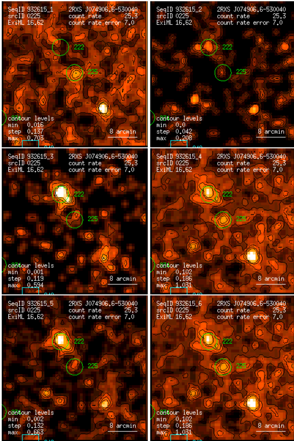
Figure 225: RASS 932615: detection 0225: band rate images, Gaussian filter: (1) PSPC channels 11 – 41, (2) 52 – 90, (3) 91 – 201, (4) 11 – 235, (5) 52 – 201, (6) 11 – 201. Broad band rates in counts/ks. Band rate contour levels in counts/ks/arcmin 2 .
