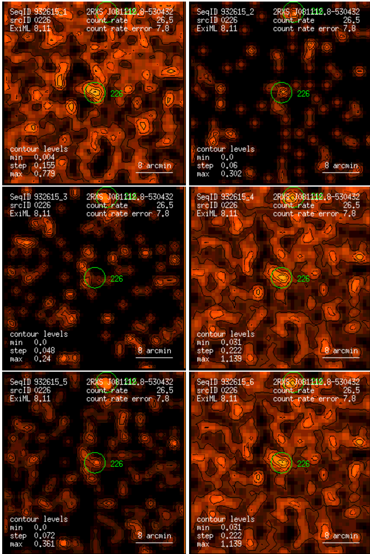
Figure 226: RASS 932615: detection 0226: band rate images, Gaussian filter: (1) PSPC channels 11 – 41, (2) 52 – 90, (3) 91 – 201, (4) 11 – 235, (5) 52 – 201, (6) 11 – 201. Broad band rates in counts/ks. Band rate contour levels in counts/ks/arcmin 2 .
