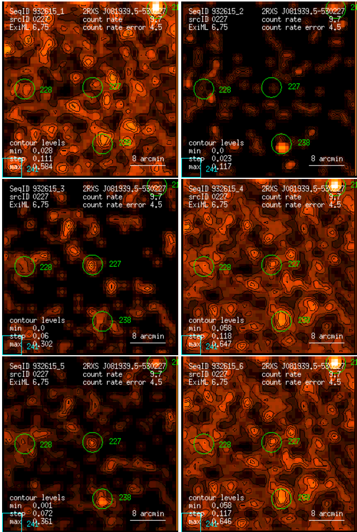
Figure 227: RASS 932615: detection 0227: band rate images, Gaussian filter: (1) PSPC channels 11 – 41, (2) 52 – 90, (3) 91 – 201, (4) 11 – 235, (5) 52 – 201, (6) 11 – 201. Broad band rates in counts/ks. Band rate contour levels in counts/ks/arcmin 2 .
