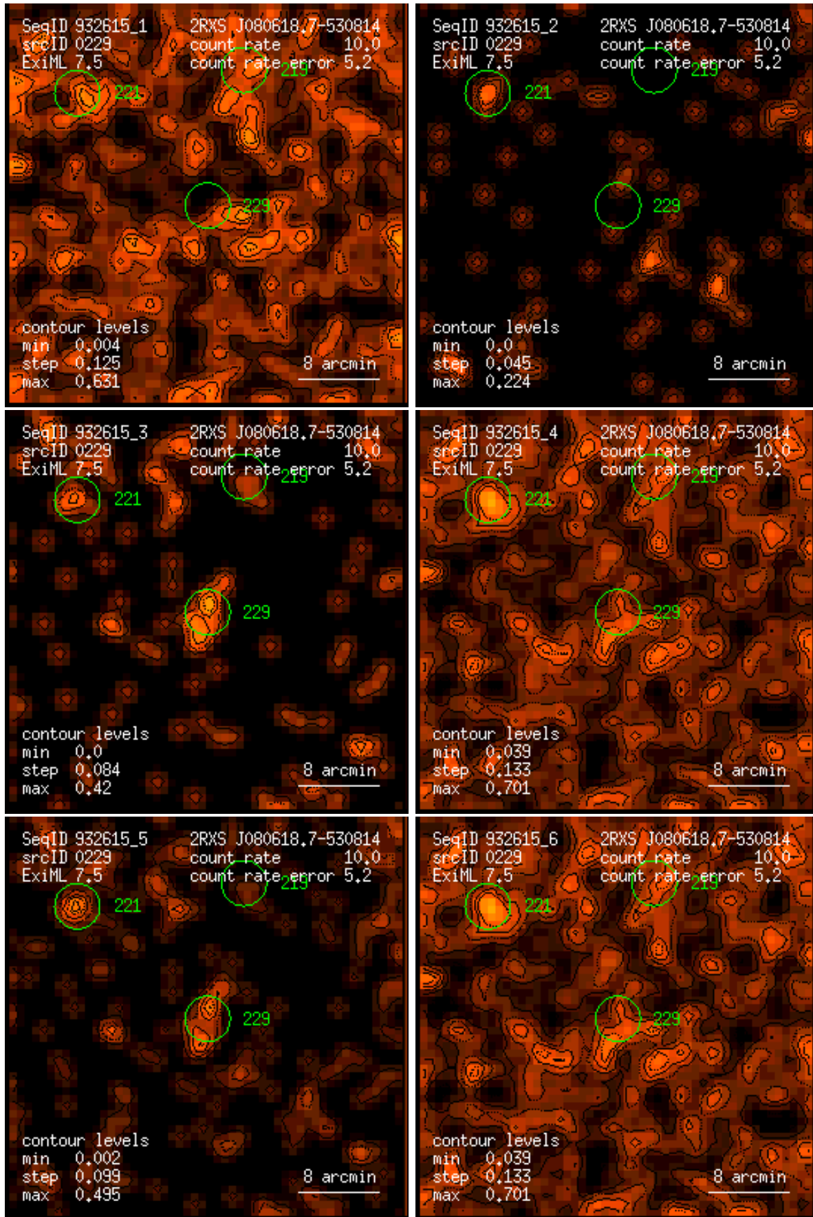
Figure 229: RASS 932615: detection 0229: band rate images, Gaussian filter: (1) PSPC channels 11 – 41, (2) 52 – 90, (3) 91 – 201, (4) 11 – 235, (5) 52 – 201, (6) 11 – 201. Broad band rates in counts/ks. Band rate contour levels in counts/ks/arcmin 2 .
