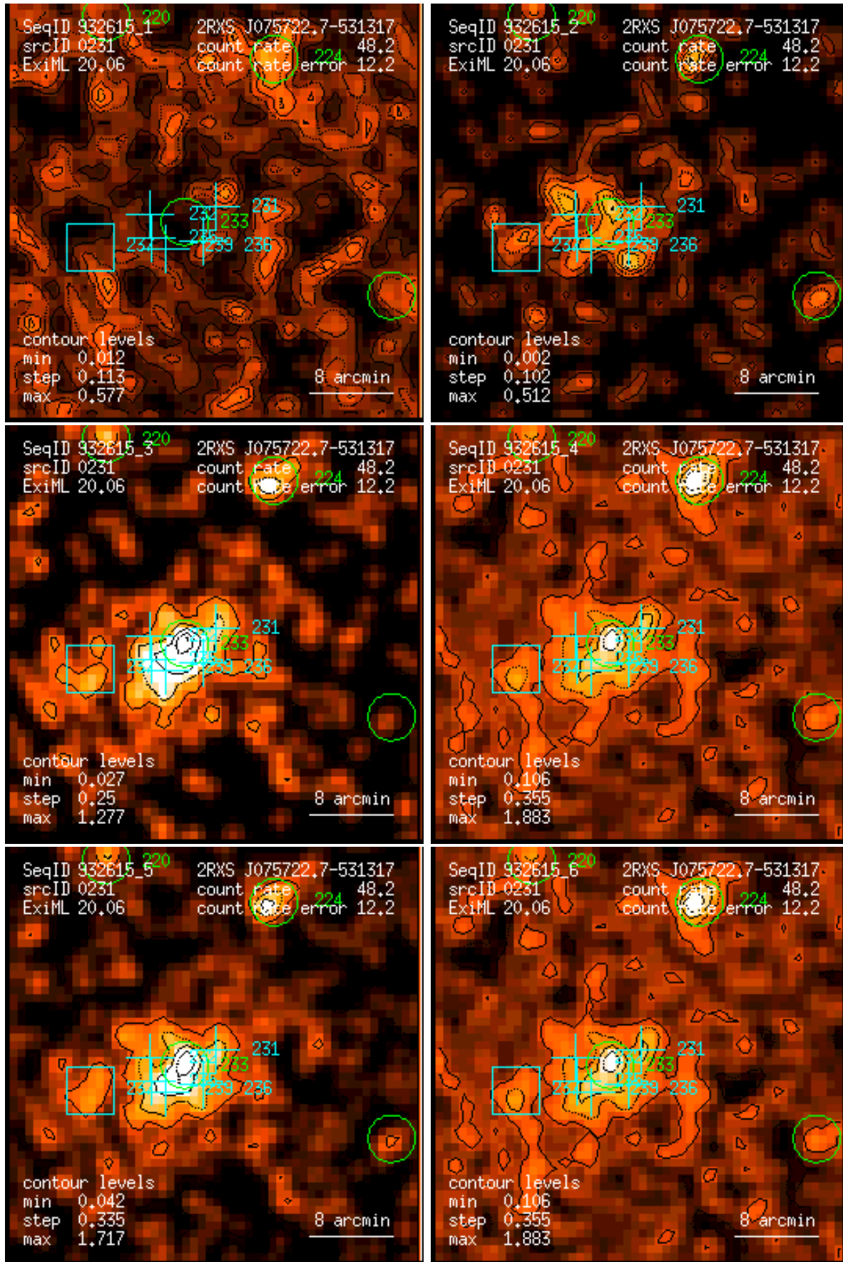
Figure 231: RASS 932615: detection 0231: band rate images, Gaussian filter: (1) PSPC channels 11 – 41, (2) 52 – 90, (3) 91 – 201, (4) 11 – 235, (5) 52 – 201, (6) 11 – 201. Broad band rates in counts/ks. Band rate contour levels in counts/ks/arcmin 2 .
