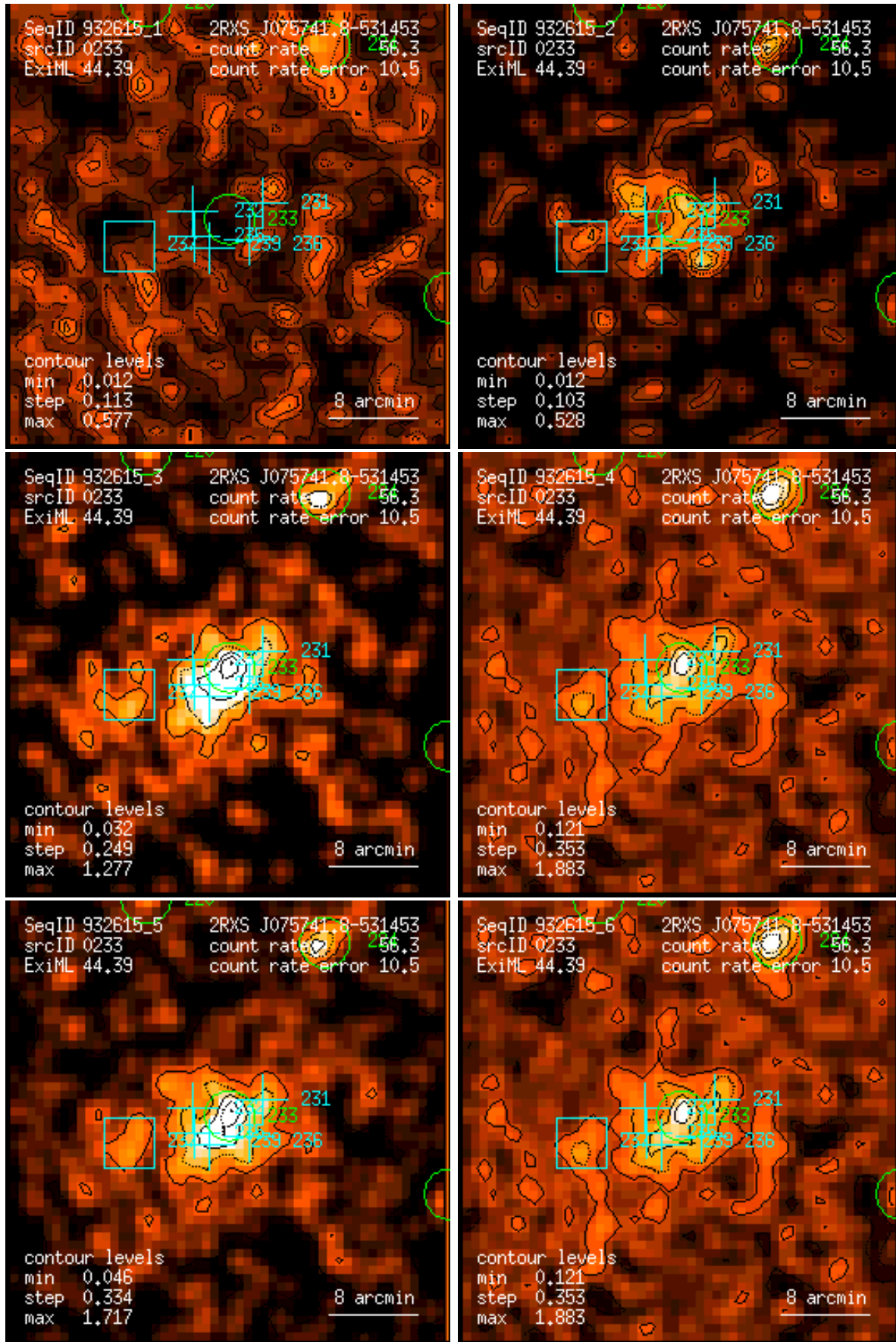
Figure 233: RASS 932615: detection 0233: band rate images, Gaussian filter: (1) PSPC channels 11 – 41, (2) 52 – 90, (3) 91 – 201, (4) 11 – 235, (5) 52 – 201, (6) 11 – 201. Broad band rates in counts/ks. Band rate contour levels in counts/ks/arcmin 2 .
