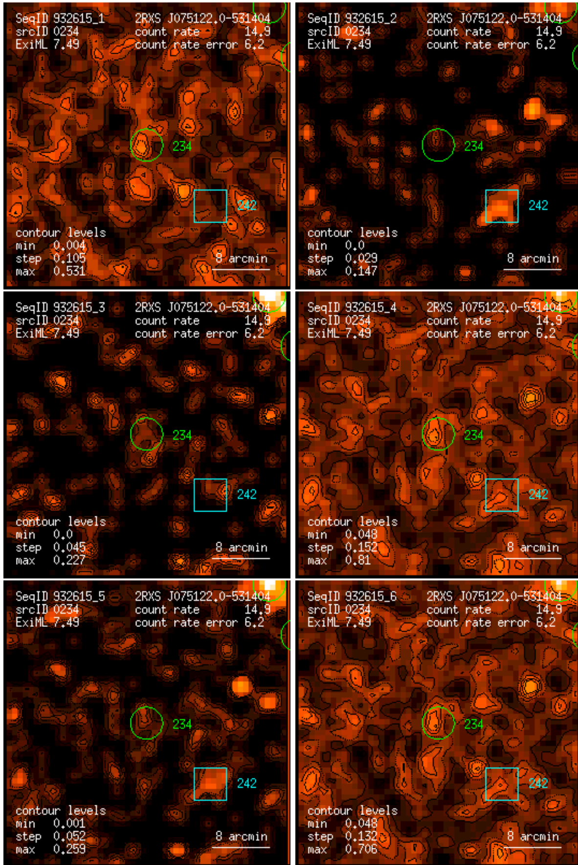
Figure 234: RASS 932615: detection 0234: band rate images, Gaussian filter: (1) PSPC channels 11 – 41, (2) 52 – 90, (3) 91 – 201, (4) 11 – 235, (5) 52 – 201, (6) 11 – 201. Broad band rates in counts/ks. Band rate contour levels in counts/ks/arcmin 2 .
