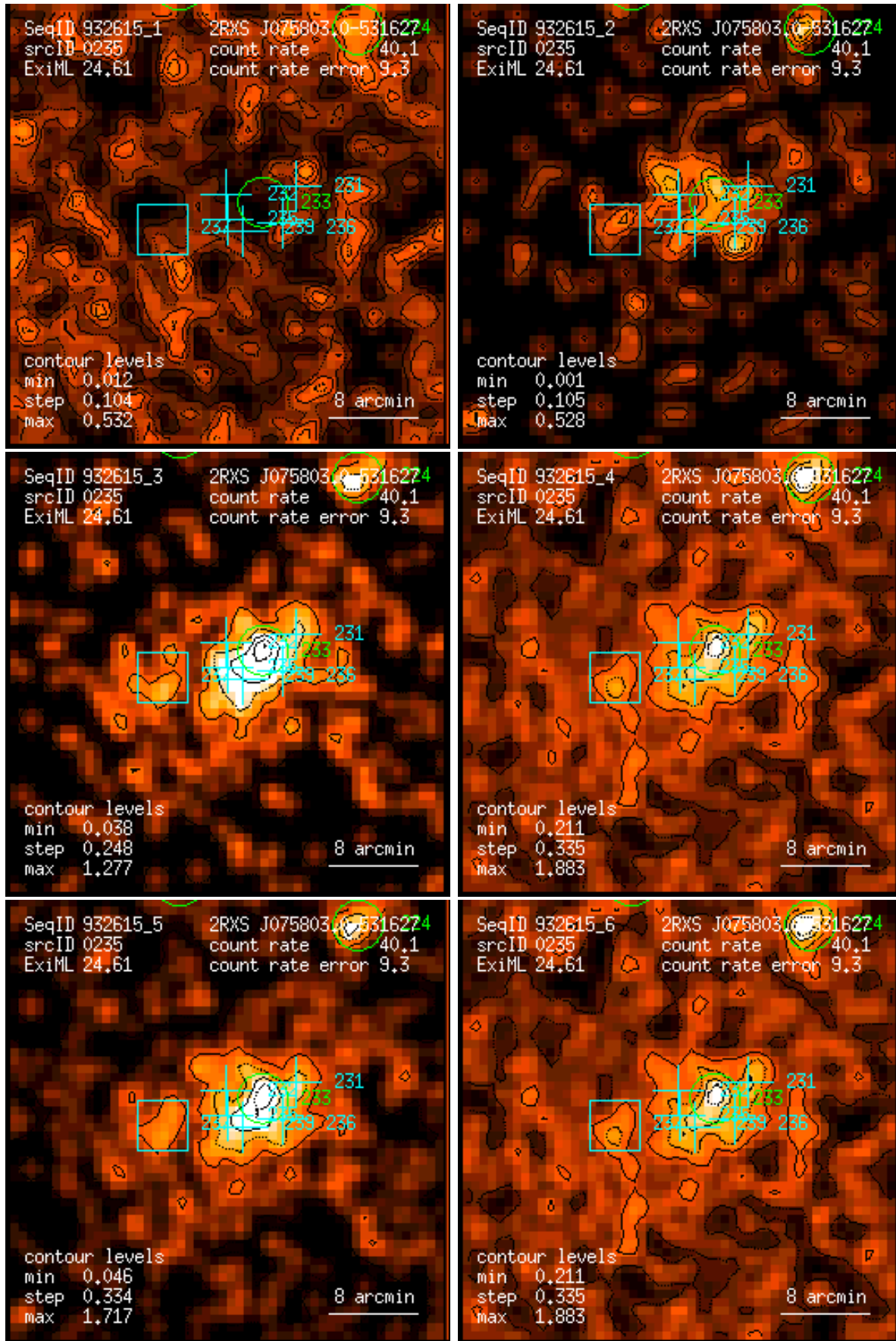
Figure 235: RASS 932615: detection 0235: band rate images, Gaussian filter: (1) PSPC channels 11 – 41, (2) 52 – 90, (3) 91 – 201, (4) 11 – 235, (5) 52 – 201, (6) 11 – 201. Broad band rates in counts/ks. Band rate contour levels in counts/ks/arcmin 2 .
