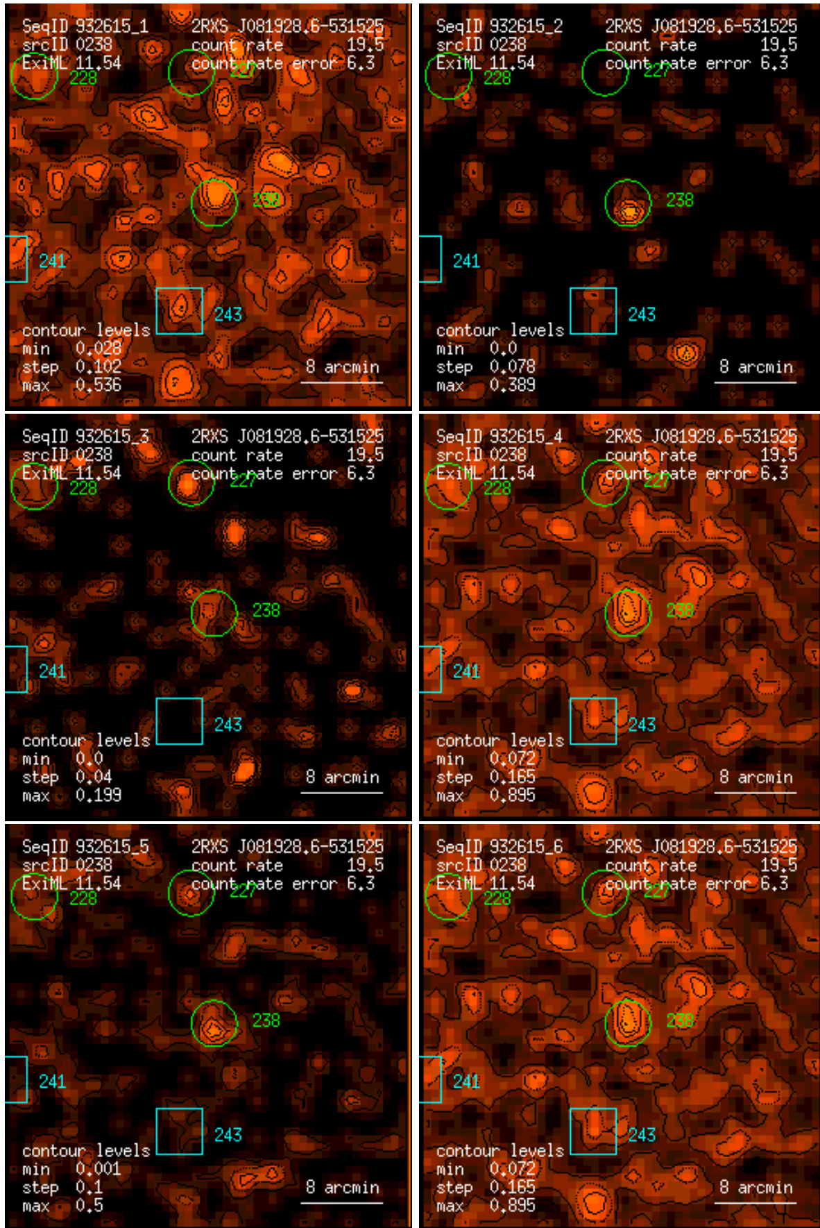
Figure 238: RASS 932615: detection 0238: band rate images, Gaussian filter: (1) PSPC channels 11 – 41, (2) 52 – 90, (3) 91 – 201, (4) 11 – 235, (5) 52 – 201, (6) 11 – 201. Broad band rates in counts/ks. Band rate contour levels in counts/ks/arcmin 2 .
