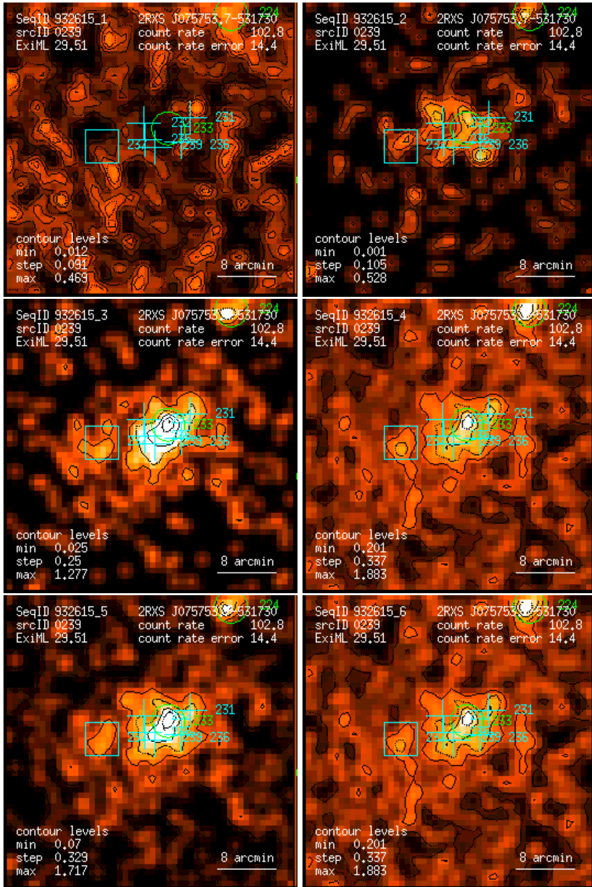
Figure 239: RASS 932615: detection 0239: band rate images, Gaussian filter: (1) PSPC channels 11 – 41, (2) 52 – 90, (3) 91 – 201, (4) 11 – 235, (5) 52 – 201, (6) 11 – 201. Broad band rates in counts/ks. Band rate contour levels in counts/ks/arcmin 2 .
