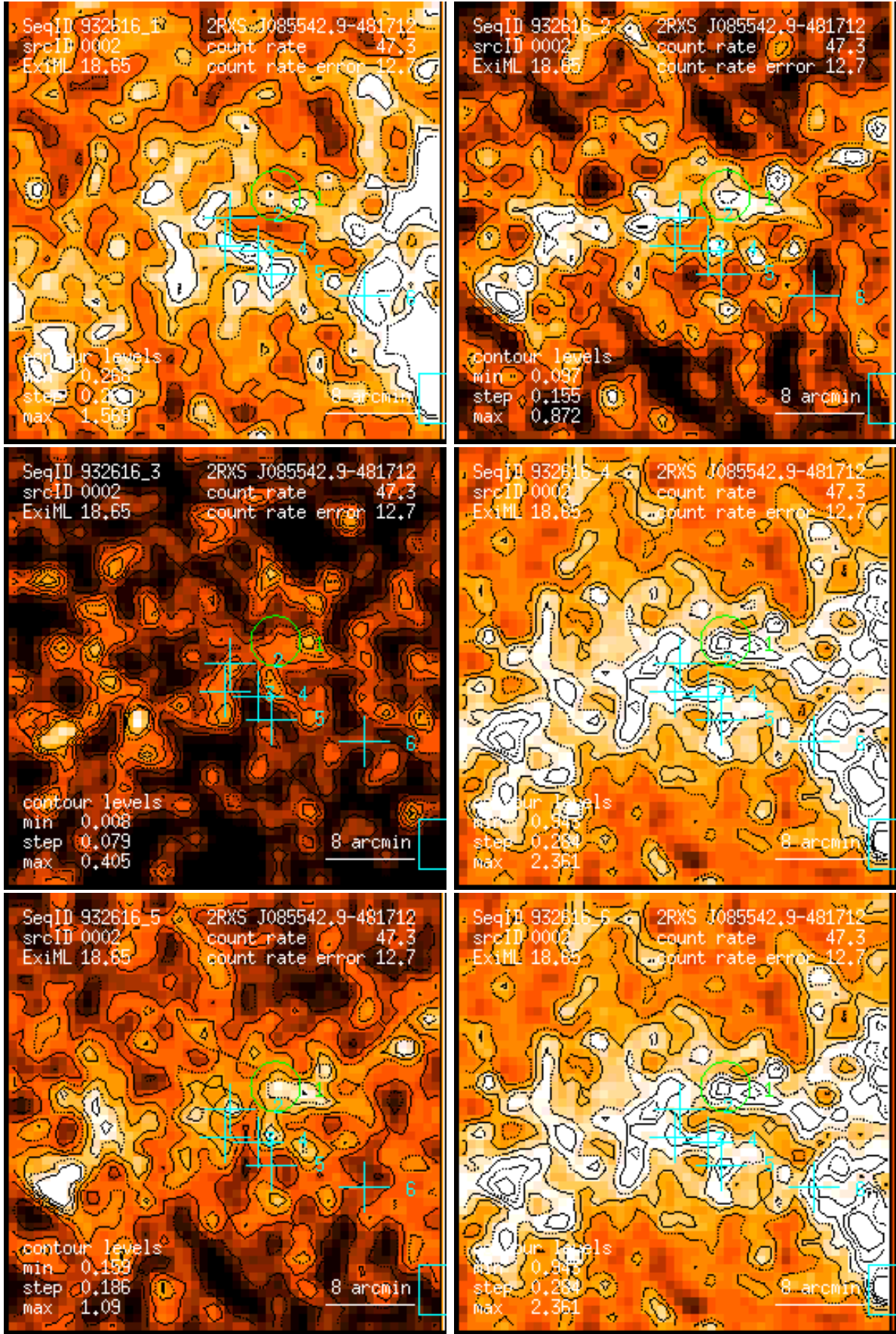
Figure 2: RASS 932616: detection 0002: band rate images, Gaussian filter: (1) PSPC channels 11 – 41, (2) 52 – 90, (3) 91 – 201, (4) 11 – 235, (5) 52 – 201, (6) 11 – 201. Broad band rates in counts/ks. Band rate contour levels in counts/ks/arcmin 2 .
