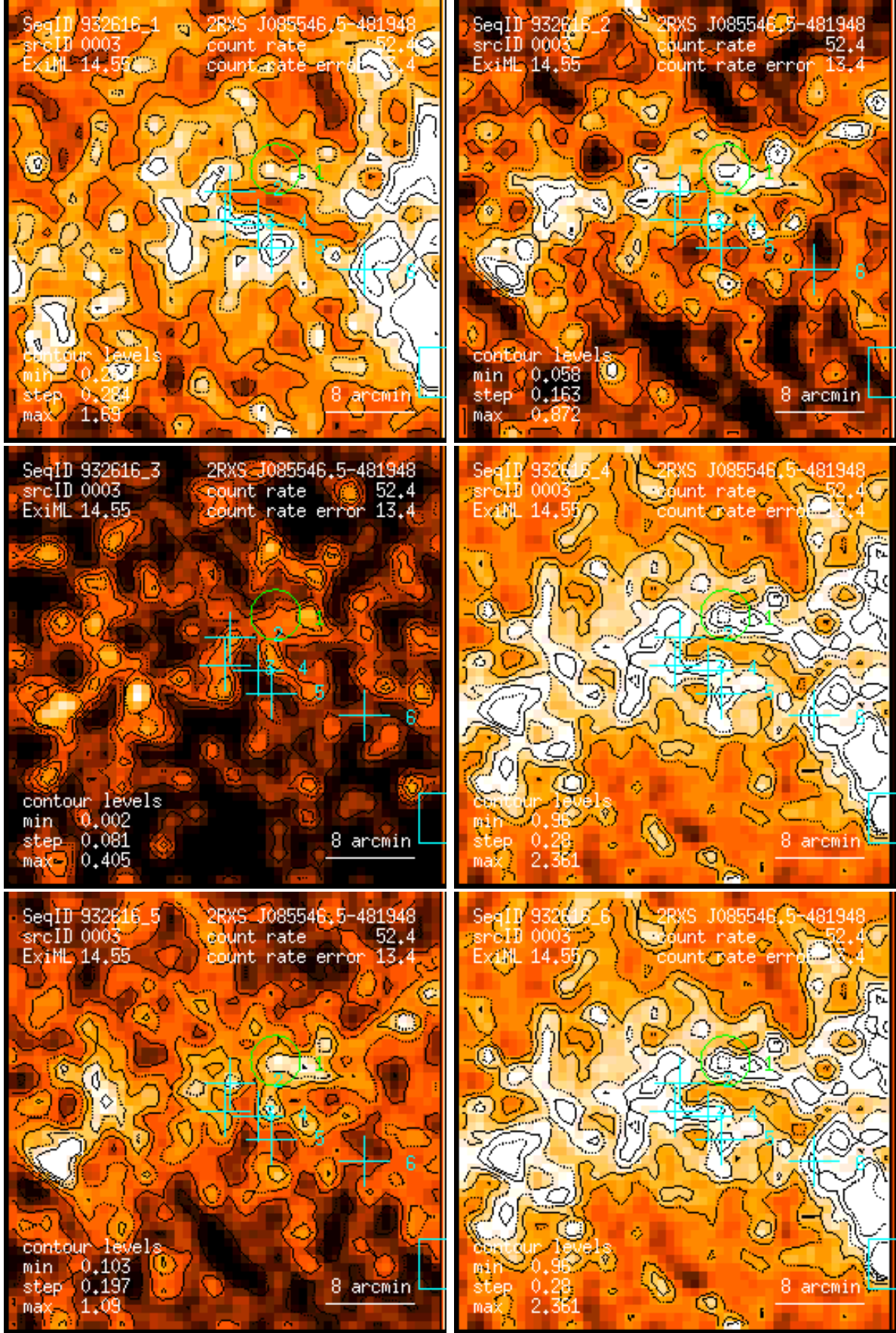
Figure 3: RASS 932616: detection 0003: band rate images, Gaussian filter: (1) PSPC channels 11 – 41, (2) 52 – 90, (3) 91 – 201, (4) 11 – 235, (5) 52 – 201, (6) 11 – 201. Broad band rates in counts/ks. Band rate contour levels in counts/ks/arcmin 2 .
