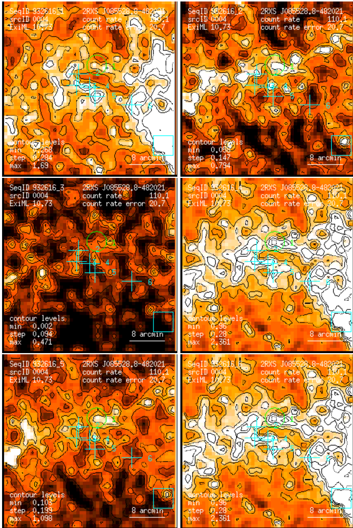
Figure 4: RASS 932616: detection 0004: band rate images, Gaussian filter: (1) PSPC channels 11 – 41, (2) 52 – 90, (3) 91 – 201, (4) 11 – 235, (5) 52 – 201, (6) 11 – 201. Broad band rates in counts/ks. Band rate contour levels in counts/ks/arcmin 2 .
