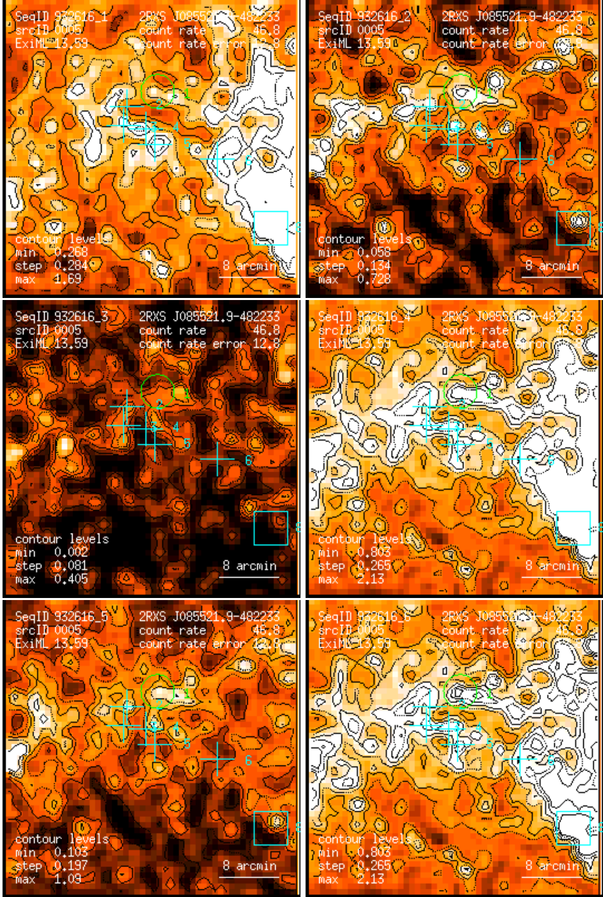
Figure 5: RASS 932616: detection 0005: band rate images, Gaussian filter: (1) PSPC channels 11 – 41, (2) 52 – 90, (3) 91 – 201, (4) 11 – 235, (5) 52 – 201, (6) 11 – 201. Broad band rates in counts/ks. Band rate contour levels in counts/ks/arcmin 2 .
