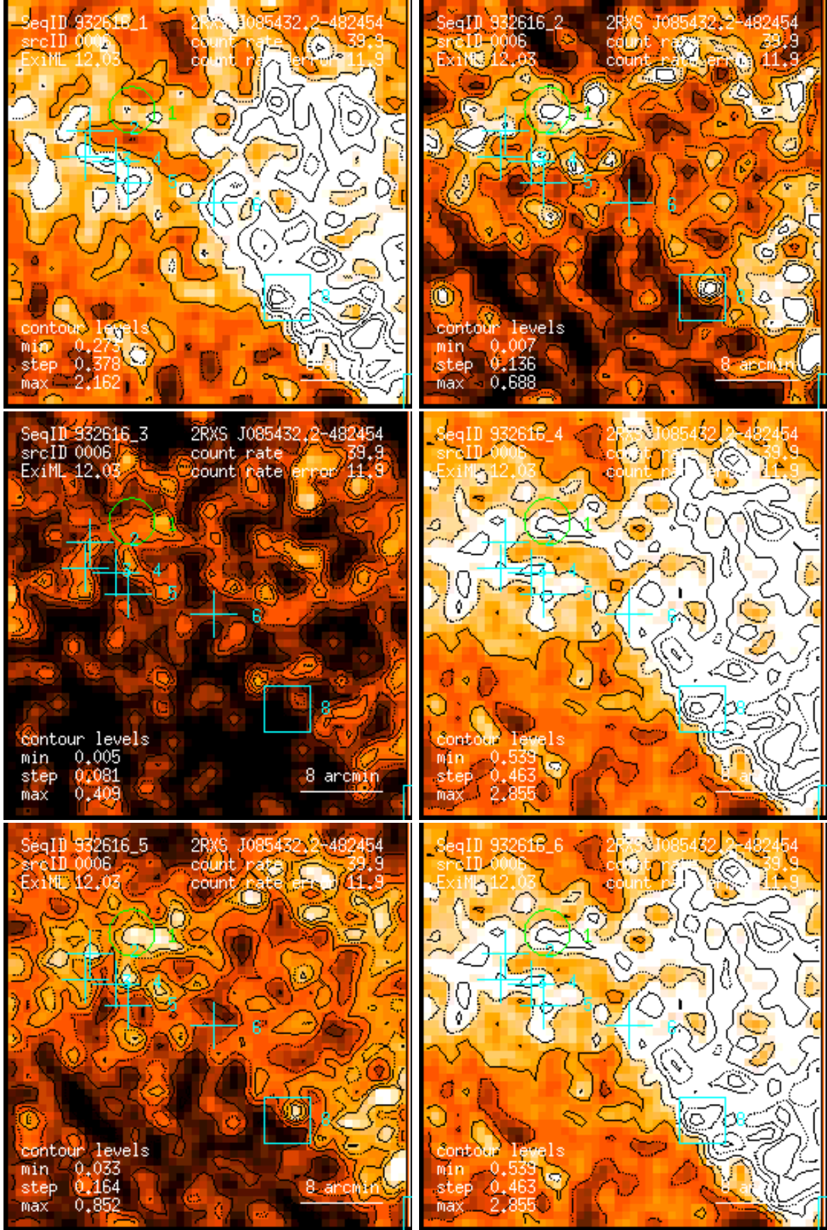
Figure 6: RASS 932616: detection 0006: band rate images, Gaussian filter: (1) PSPC channels 11 – 41, (2) 52 – 90, (3) 91 – 201, (4) 11 – 235, (5) 52 – 201, (6) 11 – 201. Broad band rates in counts/ks. Band rate contour levels in counts/ks/arcmin 2 .
