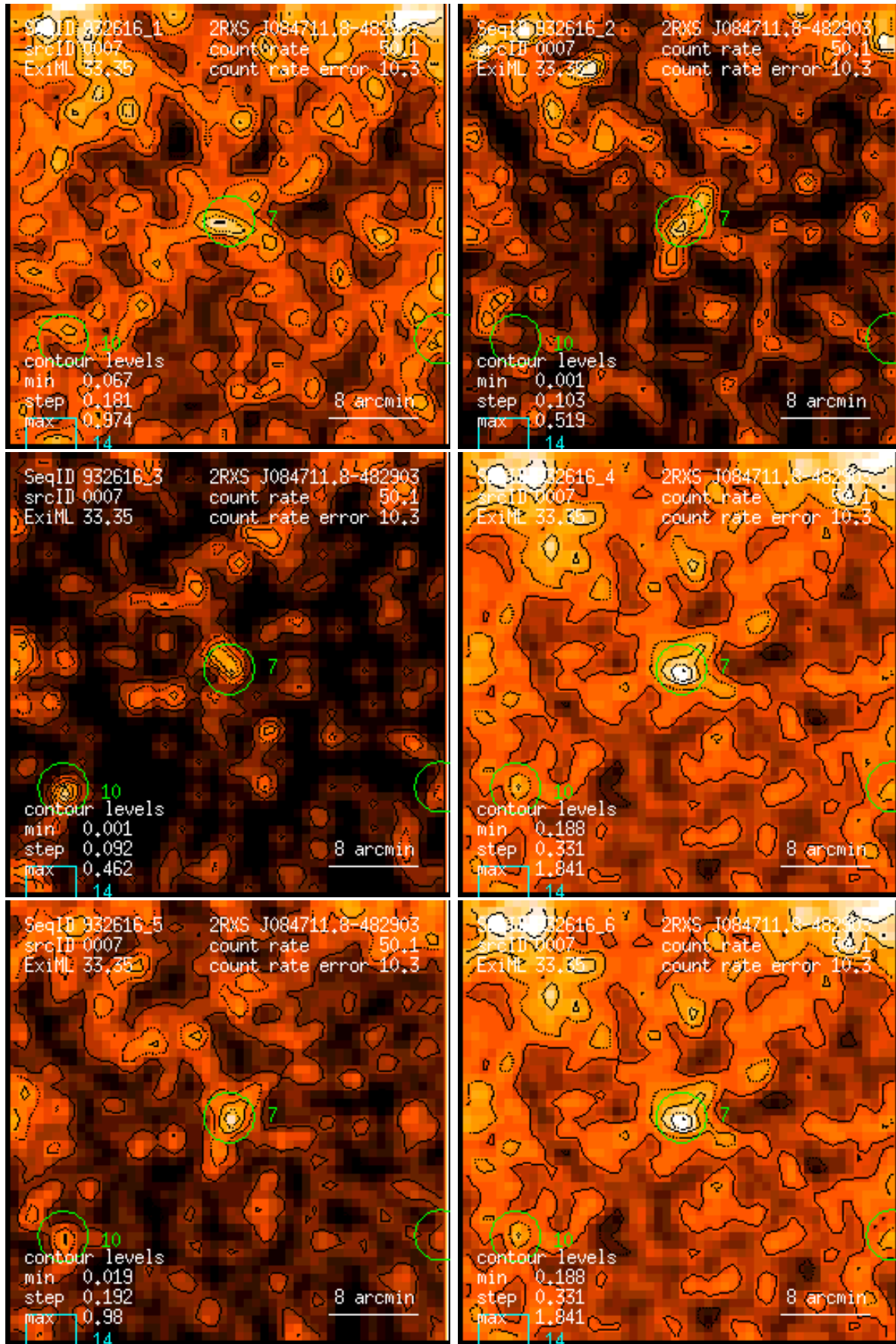
Figure 7: RASS 932616: detection 0007: band rate images, Gaussian filter: (1) PSPC channels 11 – 41, (2) 52 – 90, (3) 91 – 201, (4) 11 – 235, (5) 52 – 201, (6) 11 – 201. Broad band rates in counts/ks. Band rate contour levels in counts/ks/arcmin 2 .
