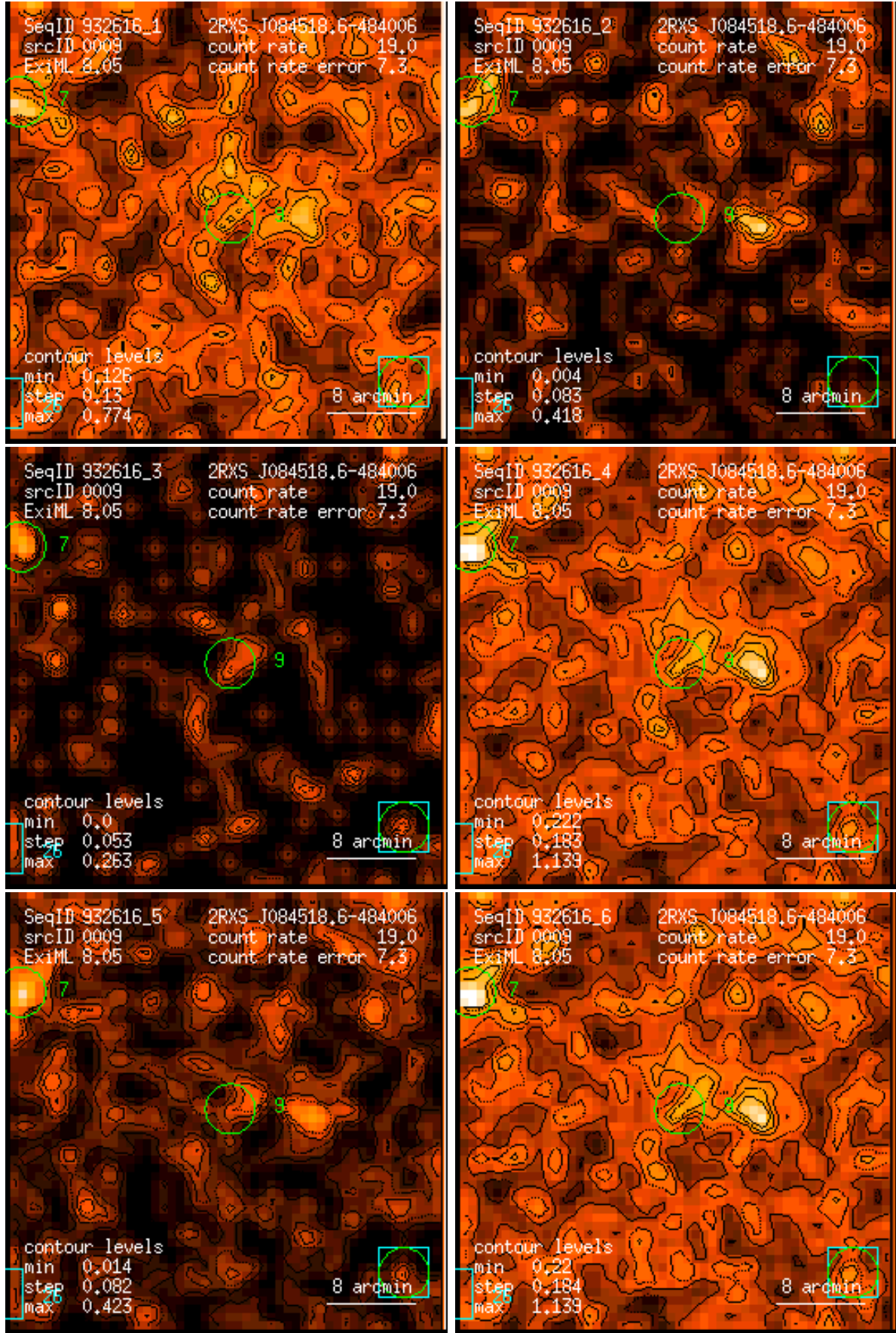
Figure 9: RASS 932616: detection 0009: band rate images, Gaussian filter: (1) PSPC channels 11 – 41, (2) 52 – 90, (3) 91 – 201, (4) 11 – 235, (5) 52 – 201, (6) 11 – 201. Broad band rates in counts/ks. Band rate contour levels in counts/ks/arcmin 2 .
