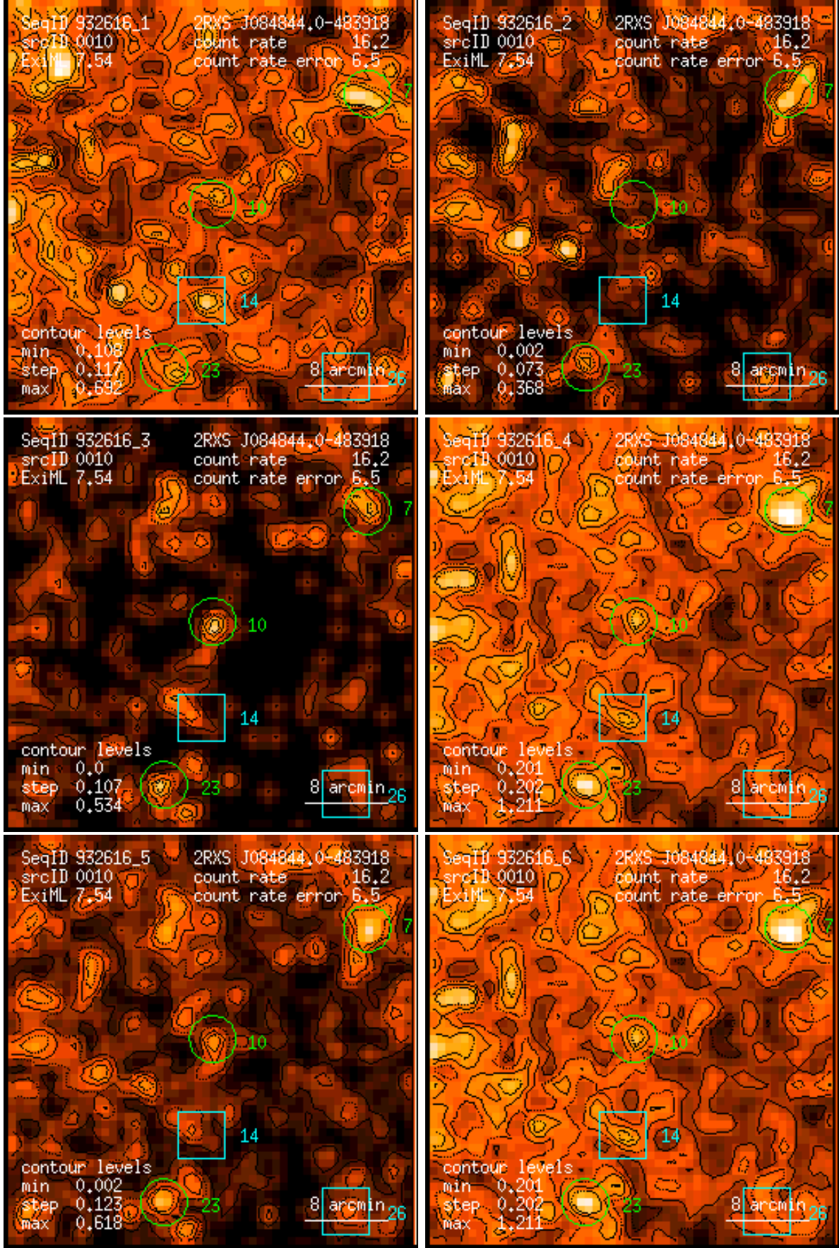
Figure 10: RASS 932616: detection 0010: band rate images, Gaussian filter: (1) PSPC channels 11 – 41, (2) 52 – 90, (3) 91 – 201, (4) 11 – 235, (5) 52 – 201, (6) 11 – 201. Broad band rates in counts/ks. Band rate contour levels in counts/ks/arcmin 2 .
