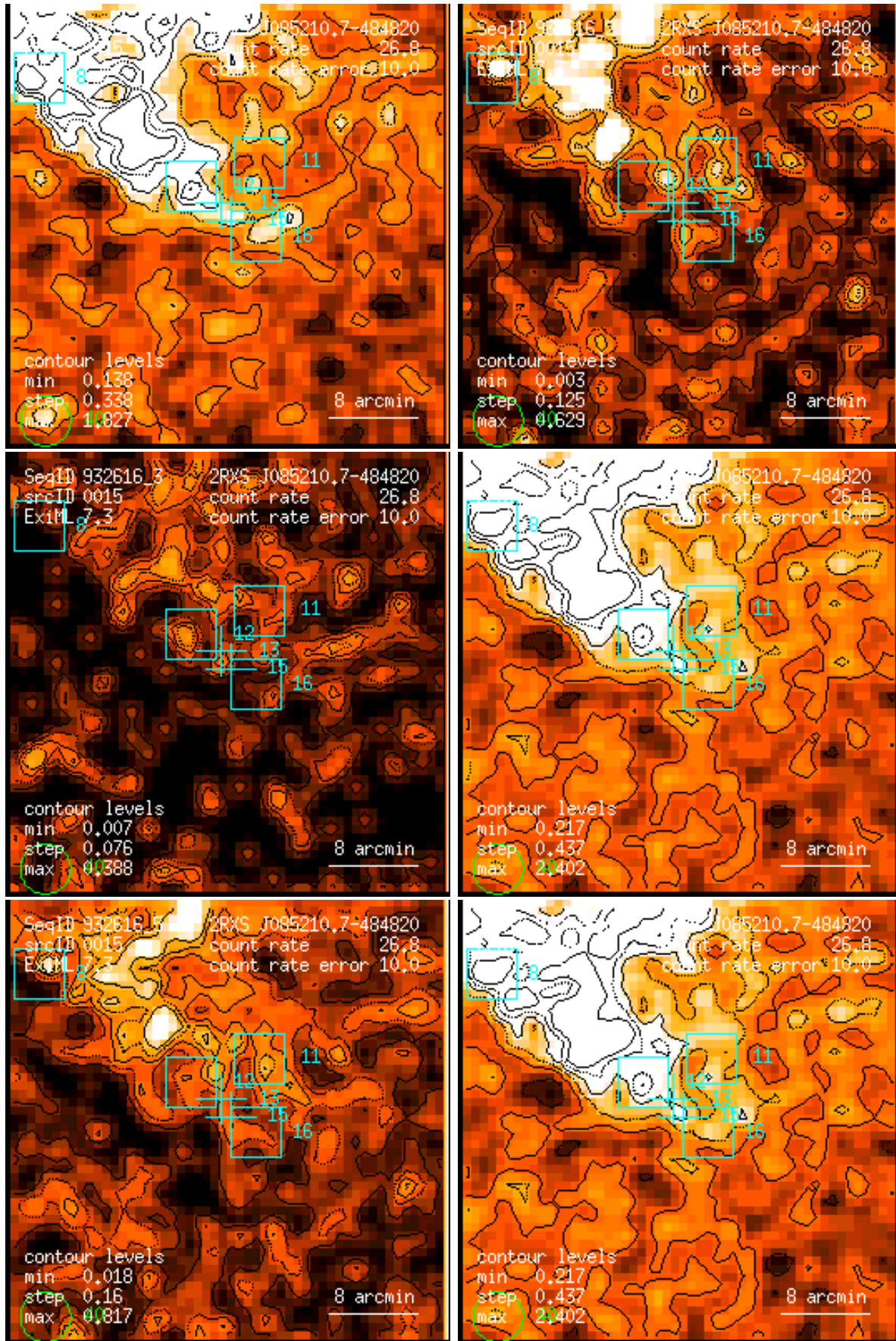
Figure 15: RASS 932616: detection 0015: band rate images, Gaussian filter: (1) PSPC channels 11 – 41, (2) 52 – 90, (3) 91 – 201, (4) 11 – 235, (5) 52 – 201, (6) 11 – 201. Broad band rates in counts/ks. Band rate contour levels in counts/ks/arcmin 2 .
