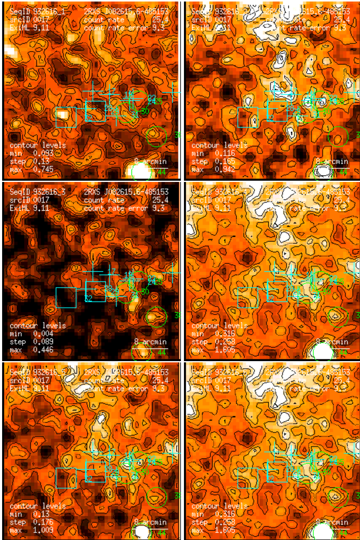
Figure 17: RASS 932616: detection 0017: band rate images, Gaussian filter: (1) PSPC channels 11 – 41, (2) 52 – 90, (3) 91 – 201, (4) 11 – 235, (5) 52 – 201, (6) 11 – 201. Broad band rates in counts/ks. Band rate contour levels in counts/ks/arcmin 2 .
