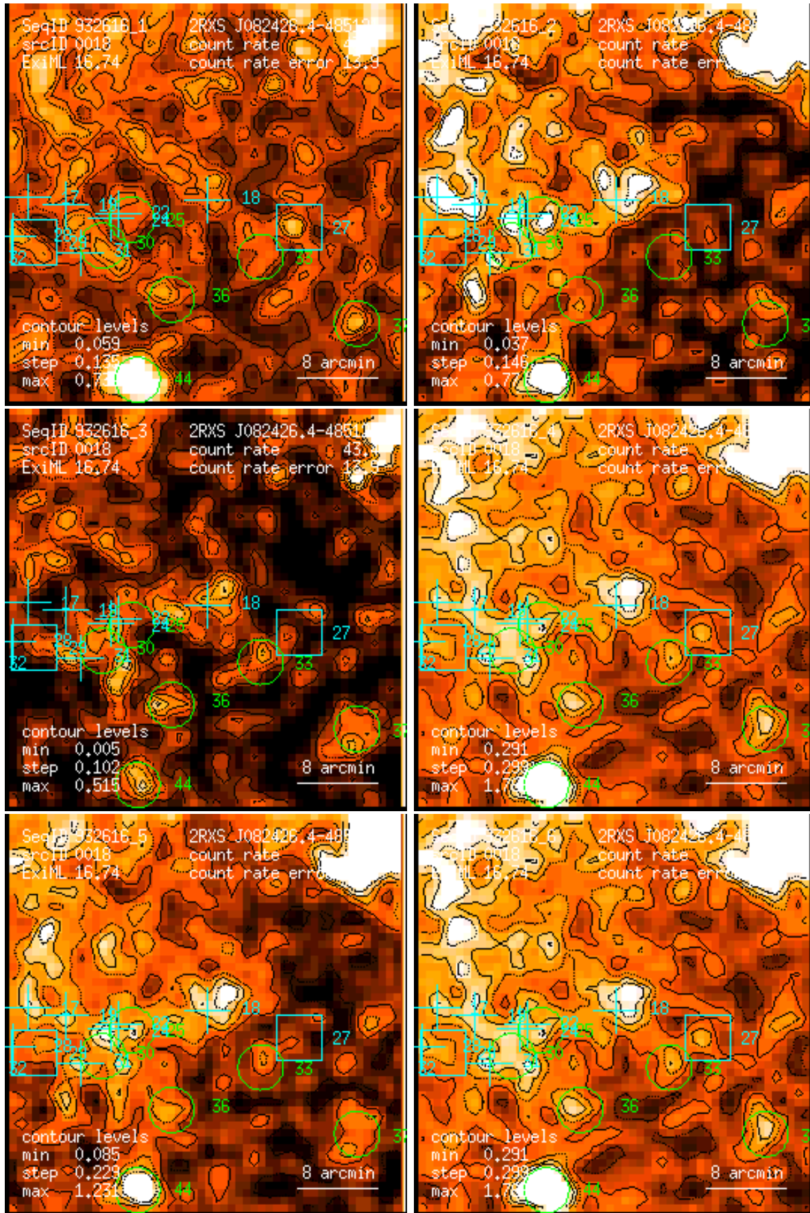
Figure 18: RASS 932616: detection 0018: band rate images, Gaussian filter: (1) PSPC channels 11 – 41, (2) 52 – 90, (3) 91 – 201, (4) 11 – 235, (5) 52 – 201, (6) 11 – 201. Broad band rates in counts/ks. Band rate contour levels in counts/ks/arcmin 2 .
