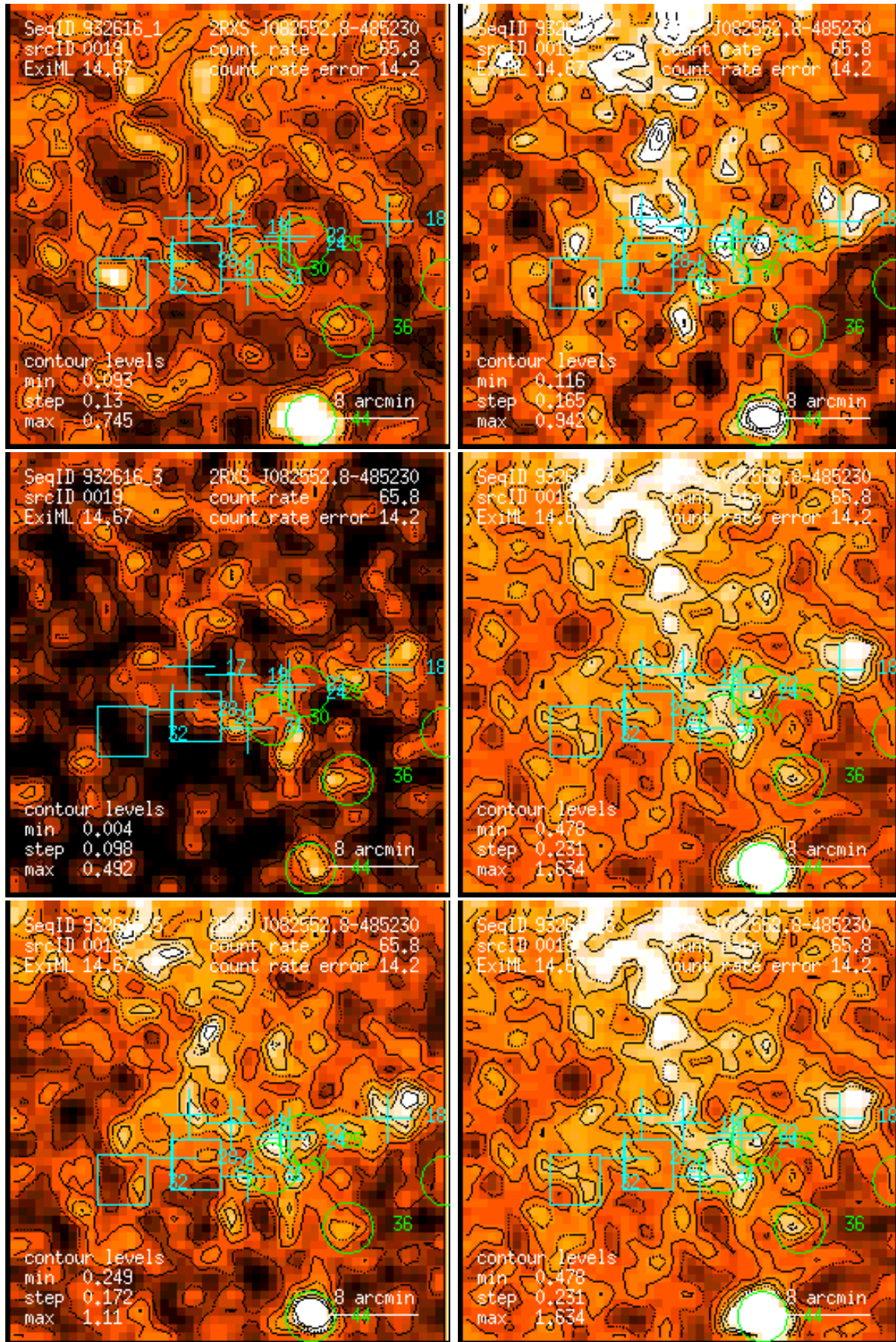
Figure 19: RASS 932616: detection 0019: band rate images, Gaussian filter: (1) PSPC channels 11 – 41, (2) 52 – 90, (3) 91 – 201, (4) 11 – 235, (5) 52 – 201, (6) 11 – 201. Broad band rates in counts/ks. Band rate contour levels in counts/ks/arcmin 2 .
