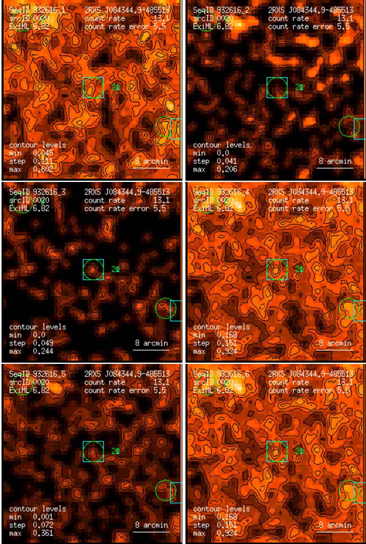
Figure 20: RASS 932616: detection 0020: band rate images, Gaussian filter: (1) PSPC channels 11 – 41, (2) 52 – 90, (3) 91 – 201, (4) 11 – 235, (5) 52 – 201, (6) 11 – 201. Broad band rates in counts/ks. Band rate contour levels in counts/ks/arcmin 2 .
